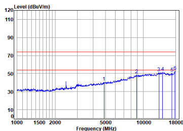
BLE_2M_TX_CH_19_Vertical
