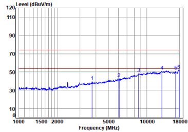
BLE_2M_TX_CH_01_Vertical
