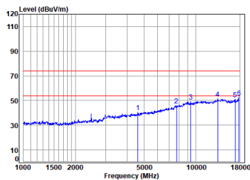
BLE_2M_TX_CH_38_Vertical
