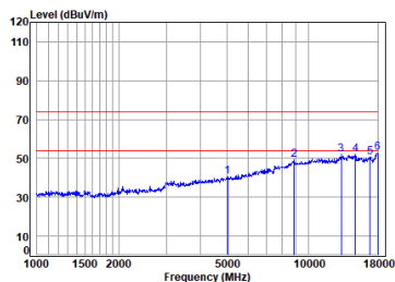
BLE_2M_TX_CH_19_Horizontal
