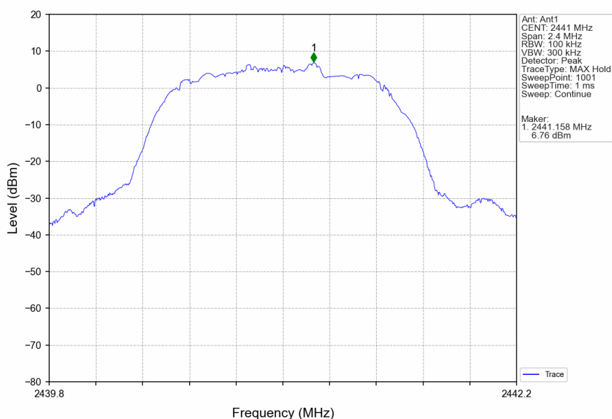
8DPSK_3DH5_MCH_2441MHz_Ant1_NTNV
