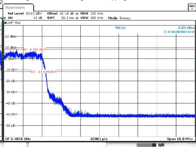
3DH5 high channel band-edge while hopping
