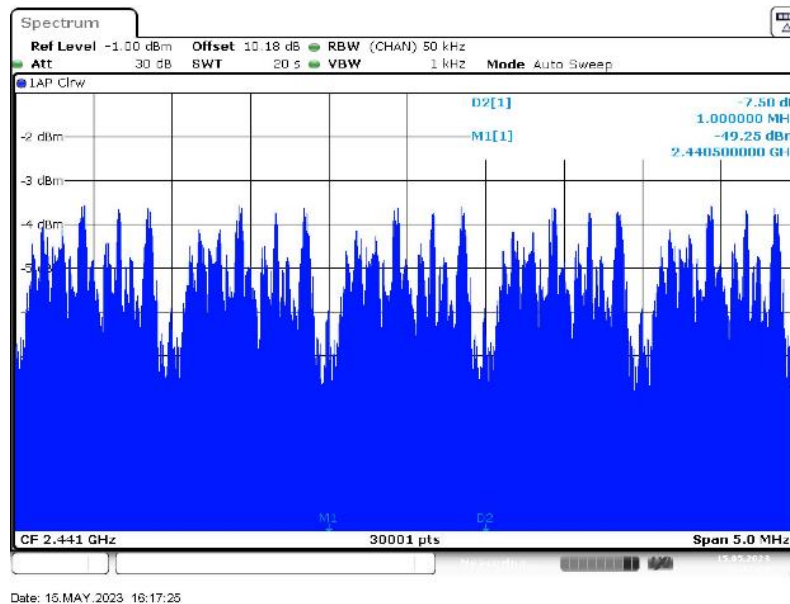
3-DH5 hopping
