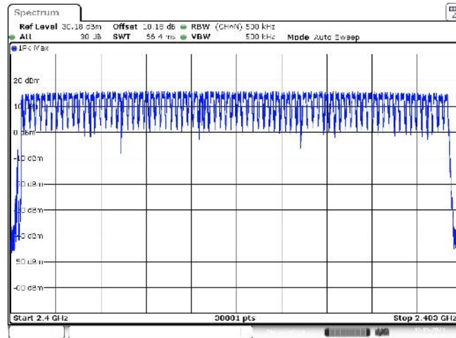
79 hopping channels active DH5
