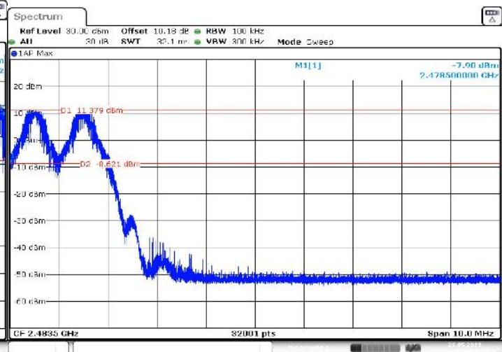
DH5 high channel band-edge while hopping
