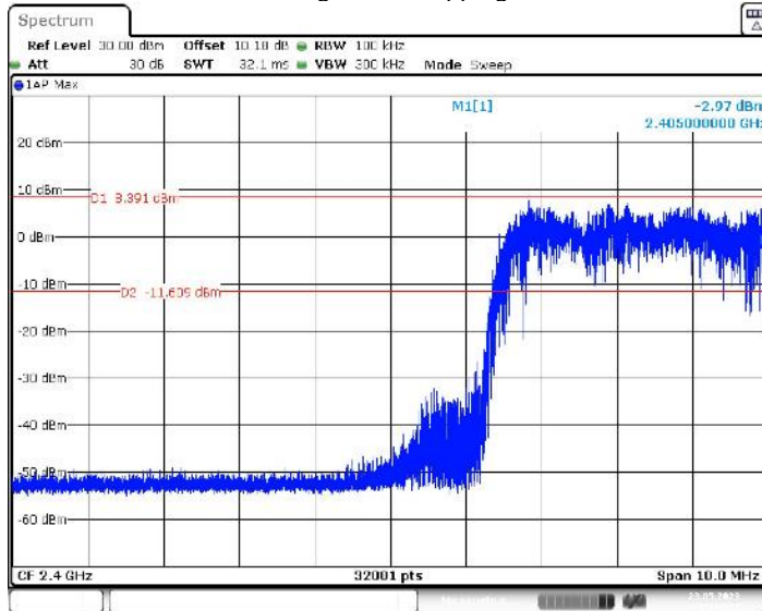
3DH5 low channel band-edge while hopping
