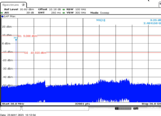
Out of band low channel (2404MHz)
