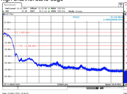
QHS-P2 high channel band-edge
