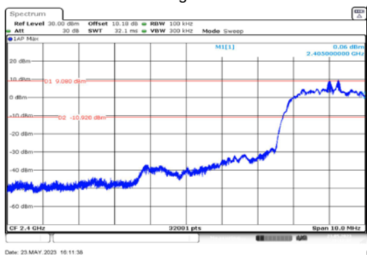
QHS-P6 low channel band-edge
