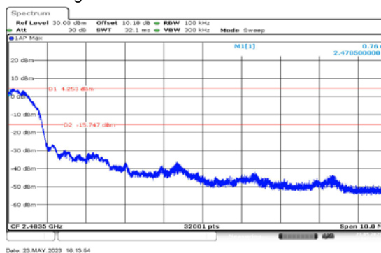
QHS-P6 high channel band-edge
