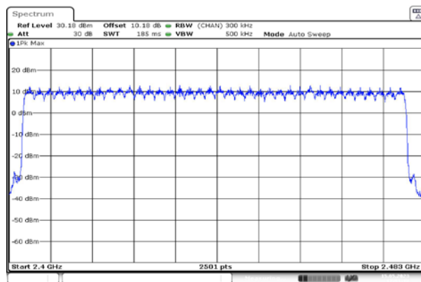
38 hopping Channels QHS-P2
