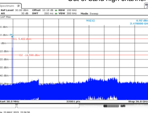
Out of band high channel (2480MHz)
