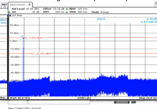
Out of band high channel (2478MHz)
