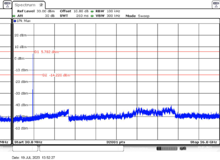
OUT-OF-BAND HIGH CHANNEL
