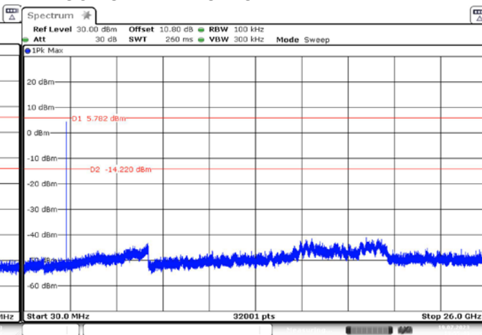
OUT-OF-BAND LOW CHANNEL
