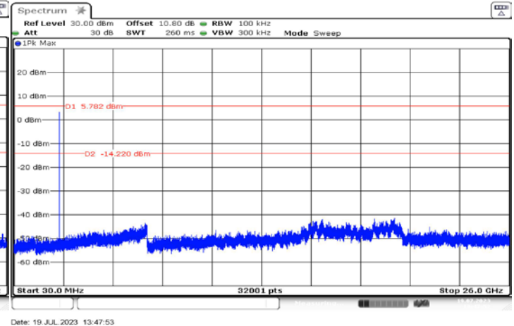
OUT-OF-BAND LOW CHANNEL
