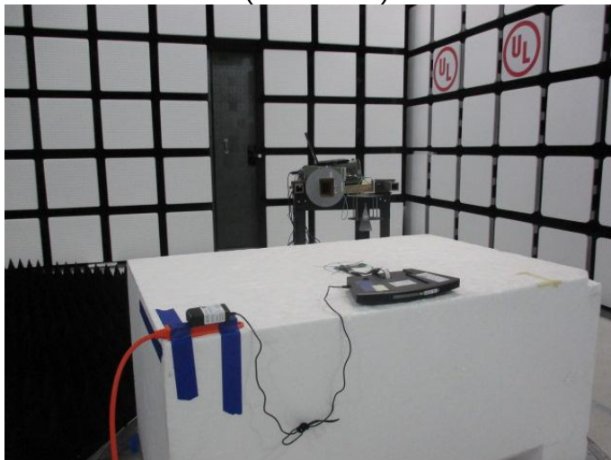
RADIATED BACK PHOTO (18-26 GHz)
