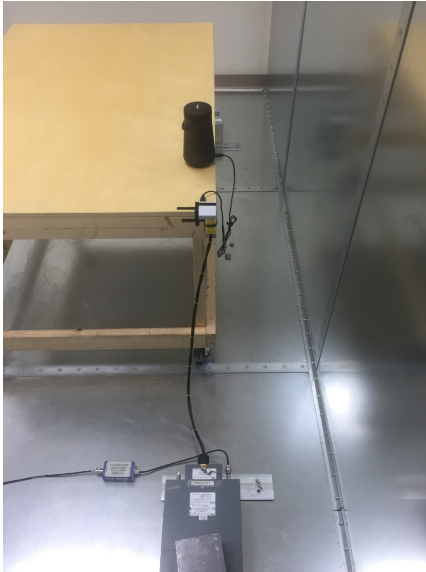
LINE CONDUCTED SIDE PHOTO
