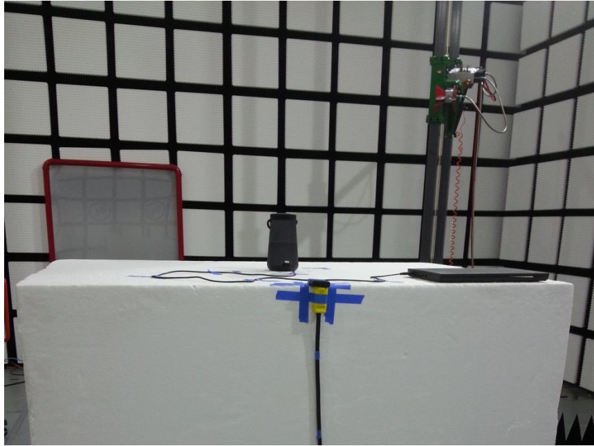
RADIATED SPURIOUS PHOTO – With Laptop
