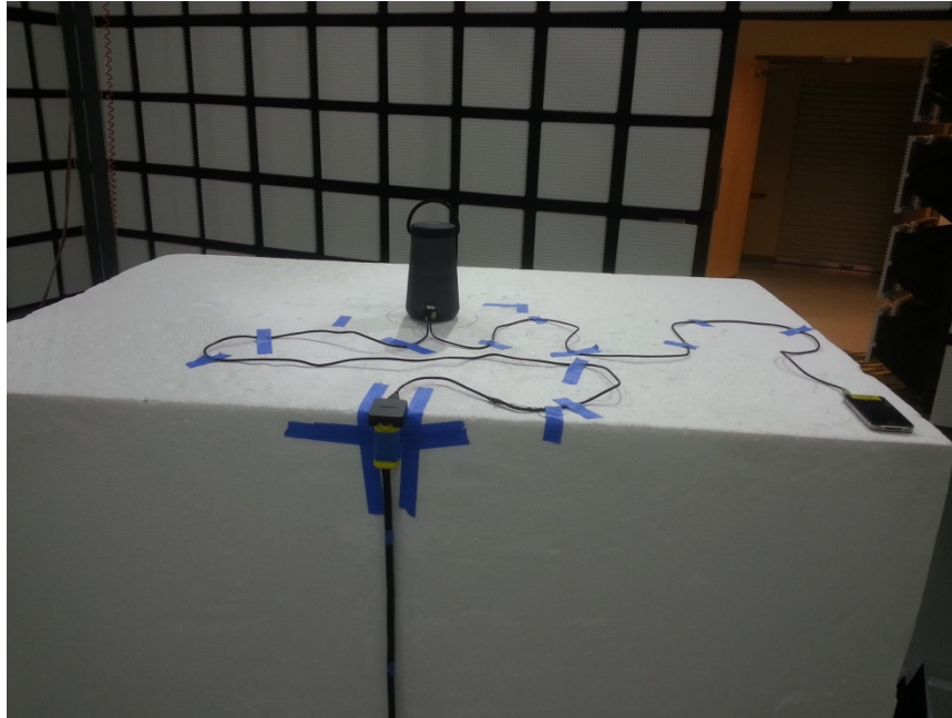
RADIATED SPURIOUS PHOTO – With Charger and Music Player
