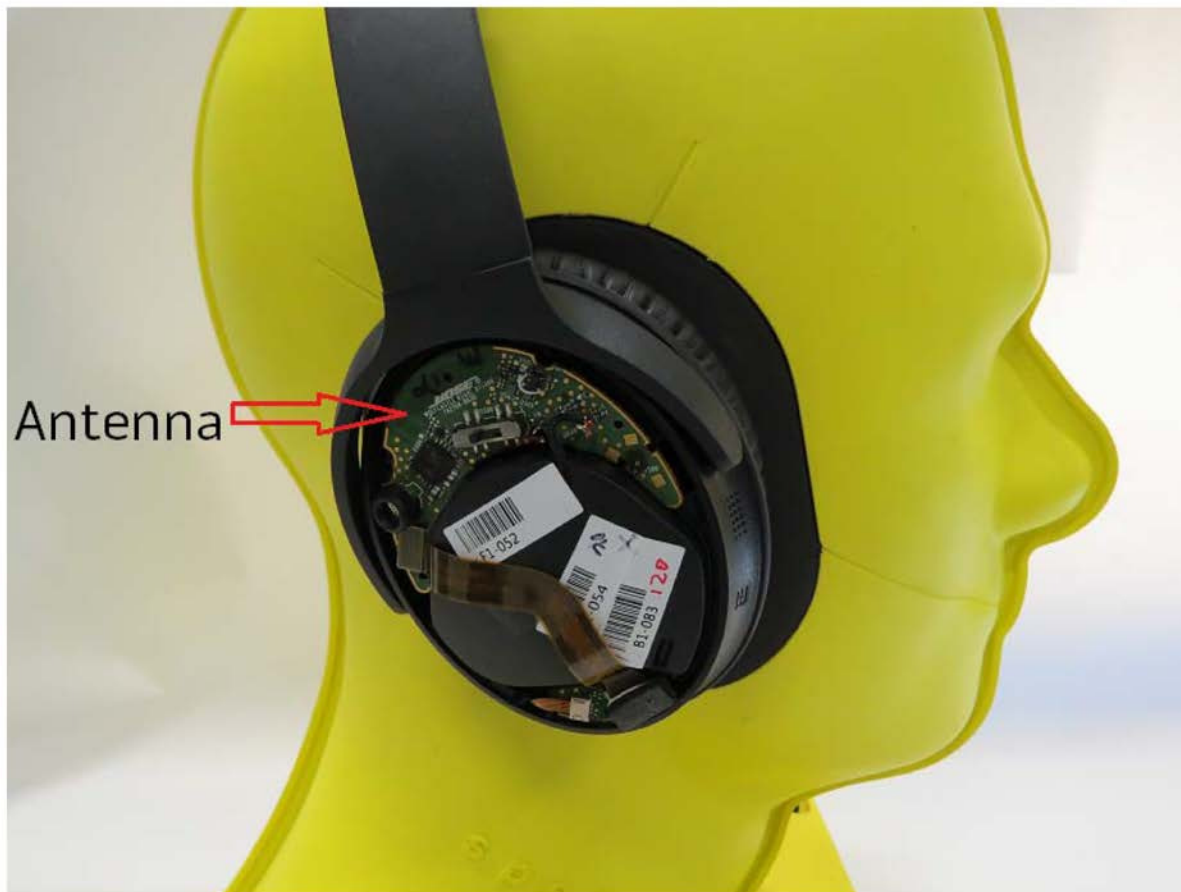
Location of Antenna with Cover Removed
