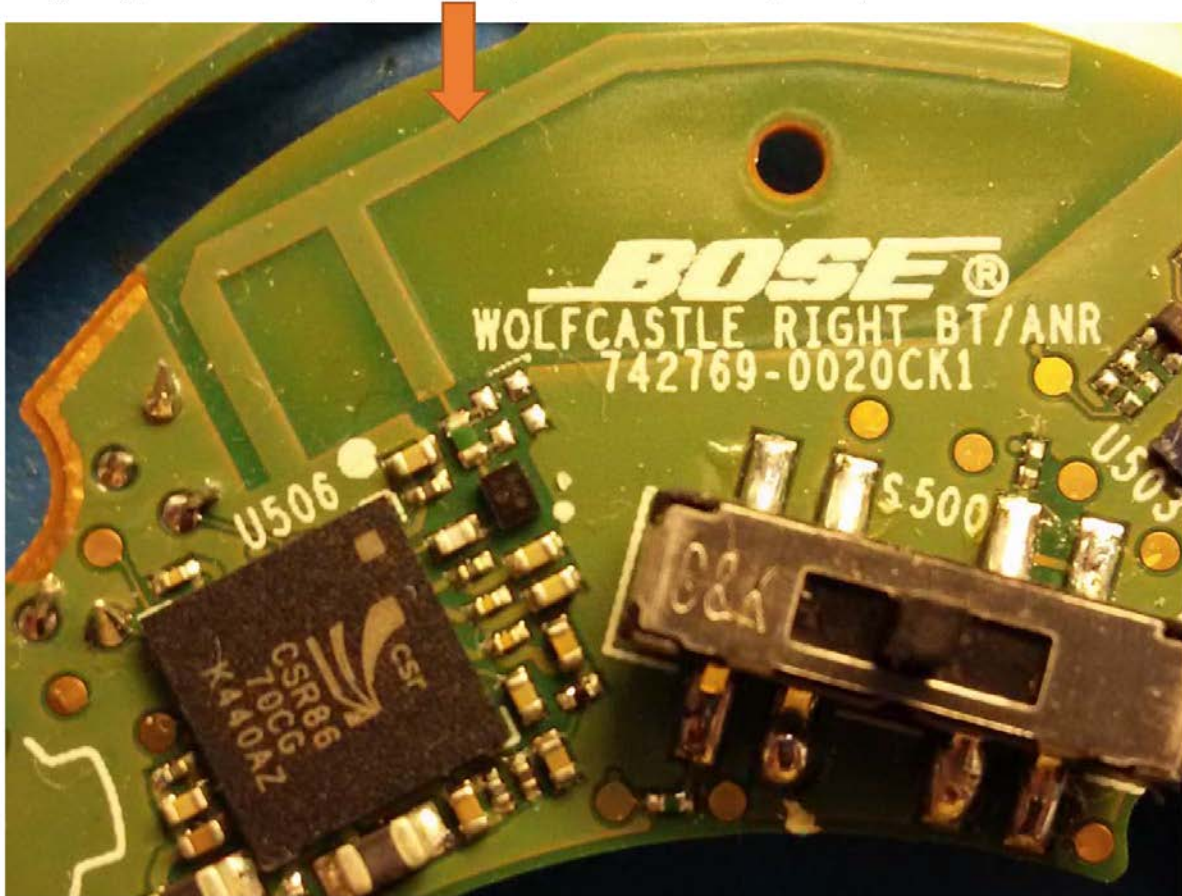
Zoomed in view of Radio PCB, w/ Antenna
