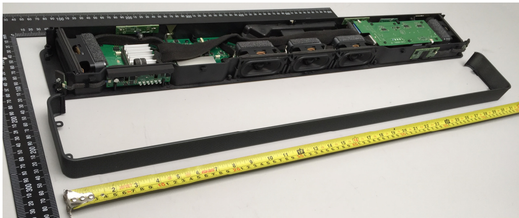
Front Metal Grille Removed
