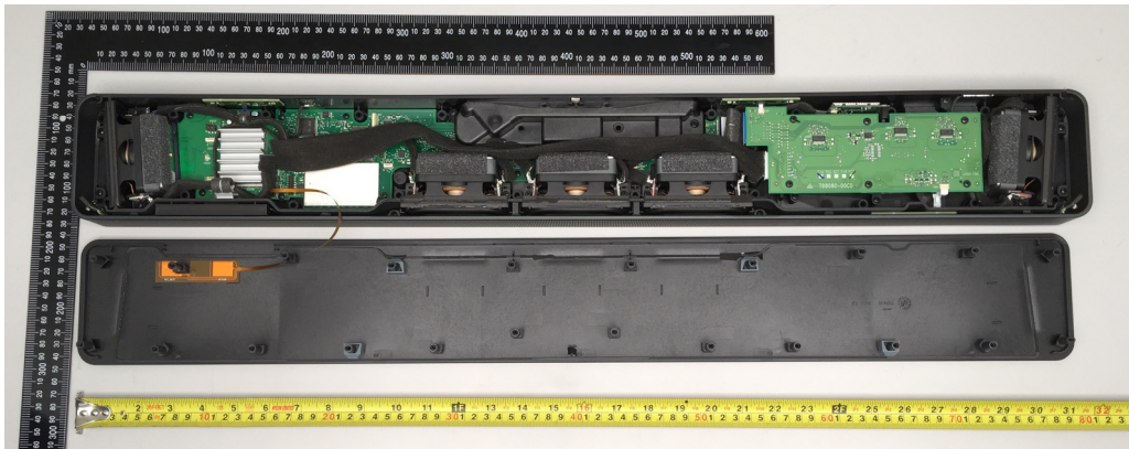
Top Cover Removed
