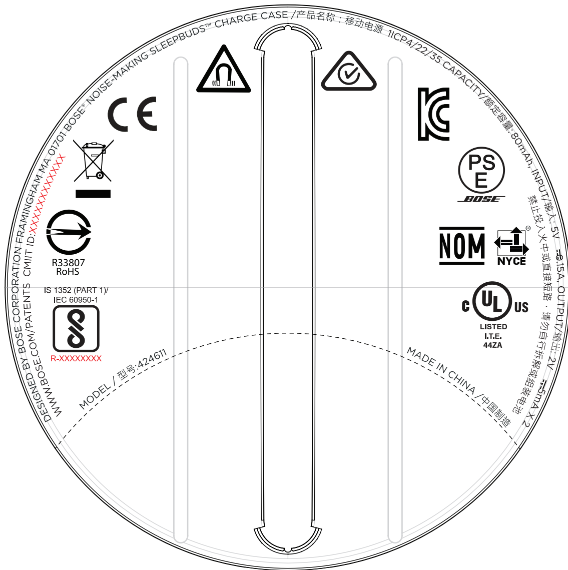
FIGURE 1.0 DRAFT MARKING PLAN (REV AN) GLOBAL SKU / LID INTERIOR 11/2/2017 OWNER: LOUIS CORREIA
