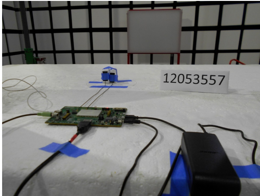
Z-AXIS EXTERNAL ANT PHOTO
