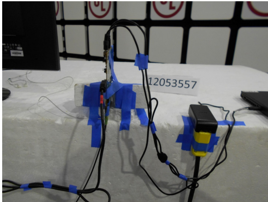
Z-AXIS PCB ANT PHOTO
