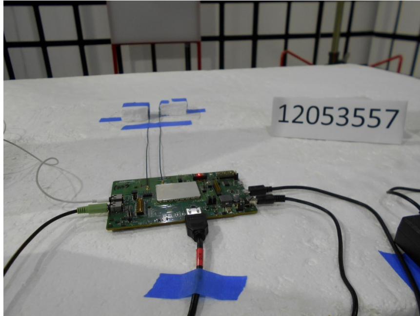
Y-AXIS EXTERNAL ANT PHOTO
