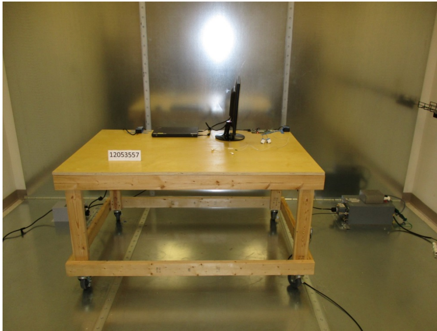
LINE CONDUCTED FRONT PHOTO EXTERNAL
