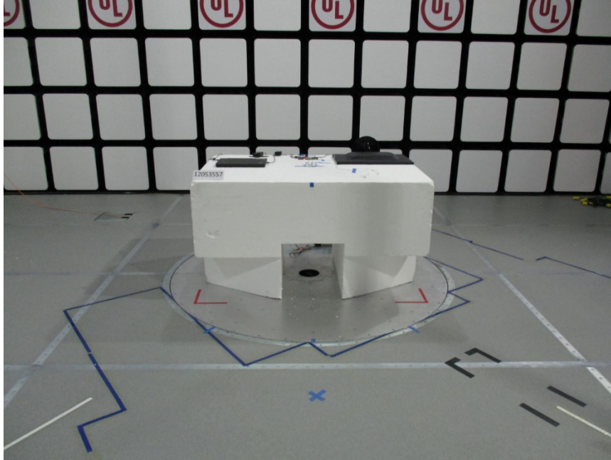
RADIATED PHOTO EXTERNAL ANT (BELOW 1 GHz)
