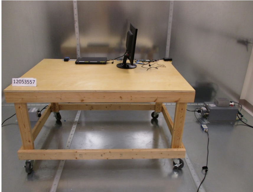
LINE CONDUCTED FRONT PHOTO PCB
