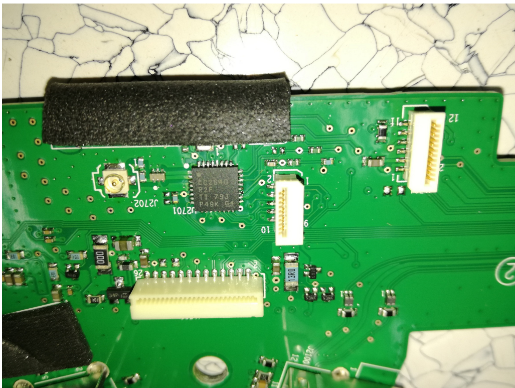
RF part
