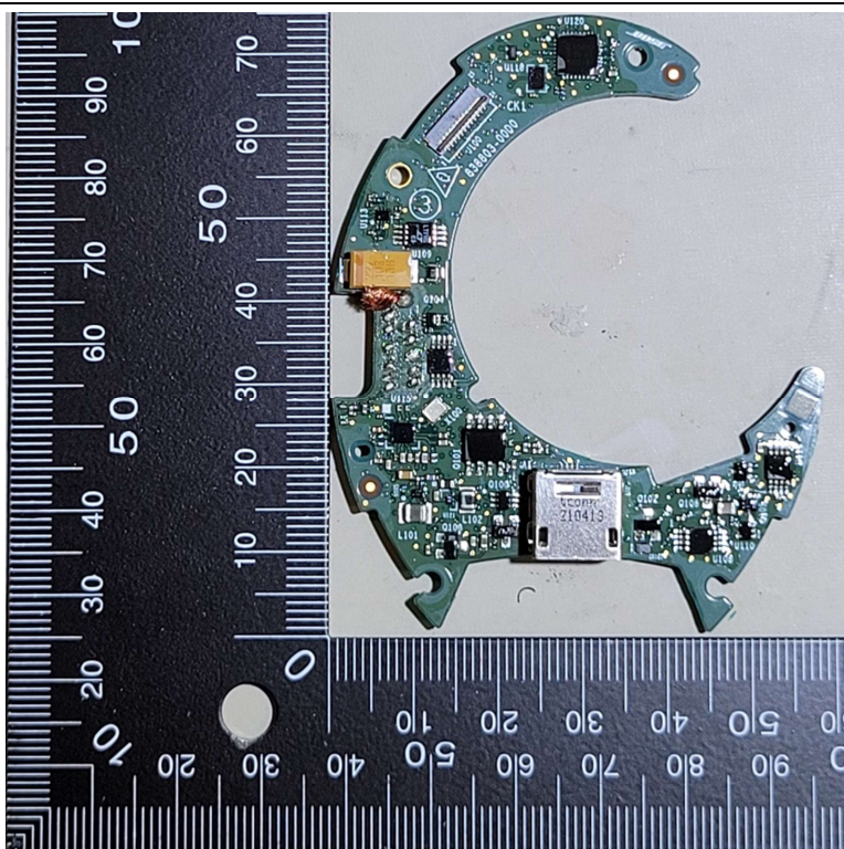
Left Earcup – Top
