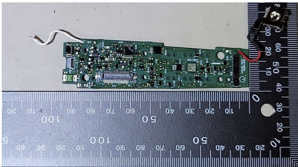
Control module, Audio/Power board – Top
