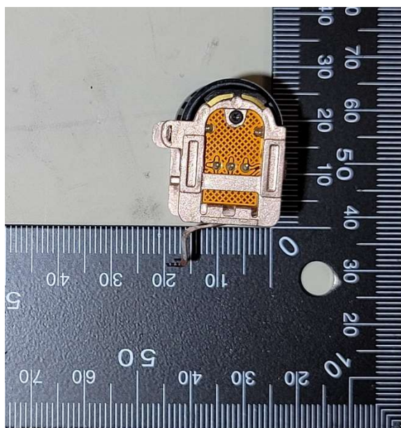
Control Module, volume wheels – Right
