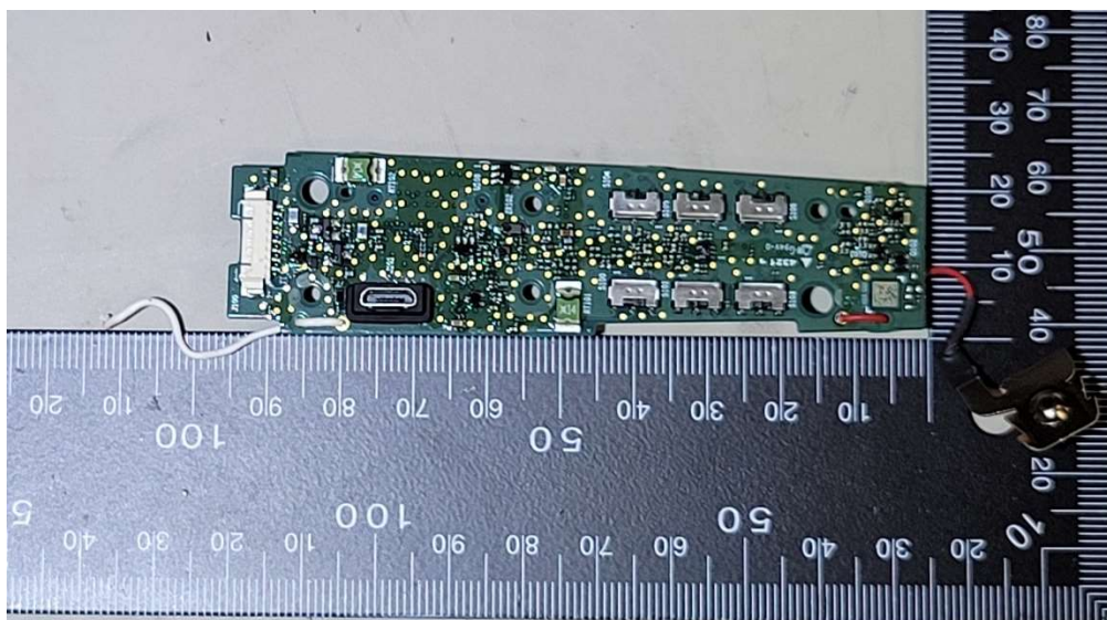
Control module, Audio/Power board – Bottom
