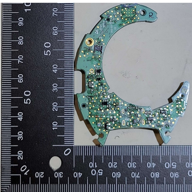
Right Earcup – Bottom
