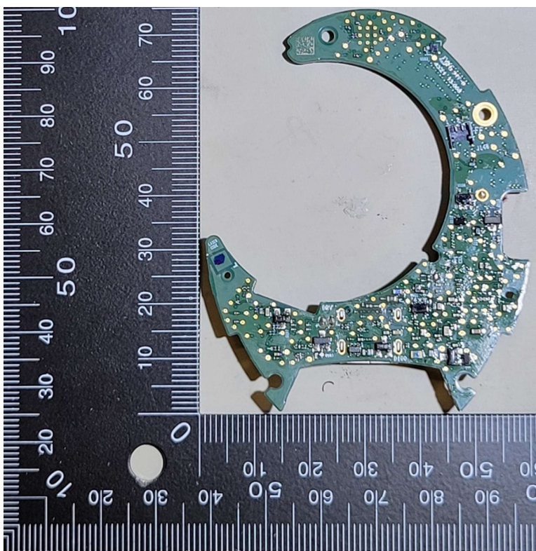
Left Earcup – Bottom
