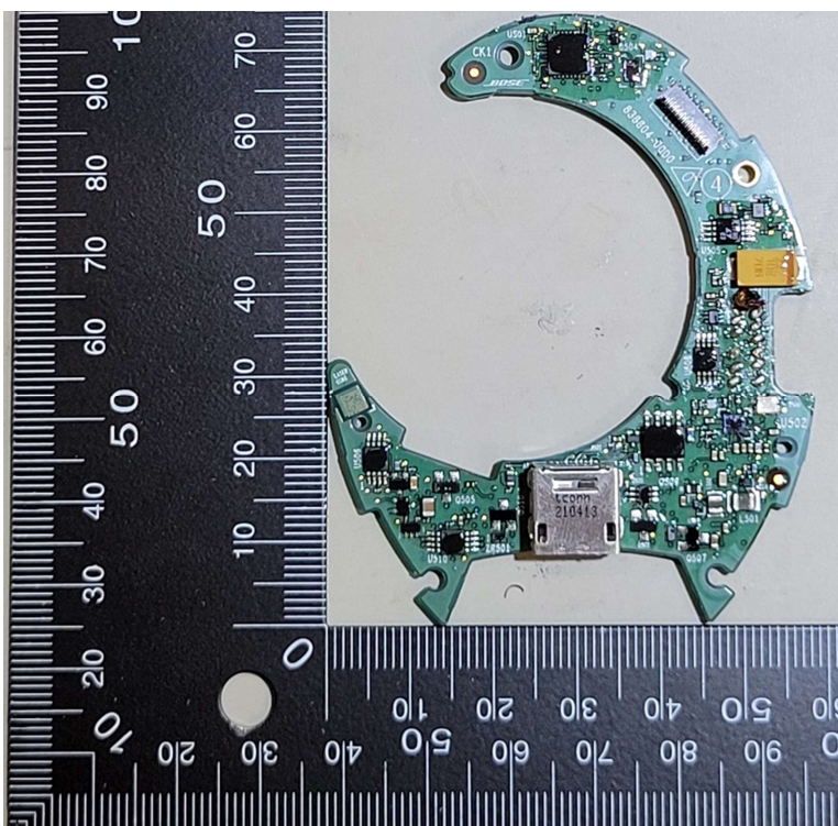
Right Earcup – Top
