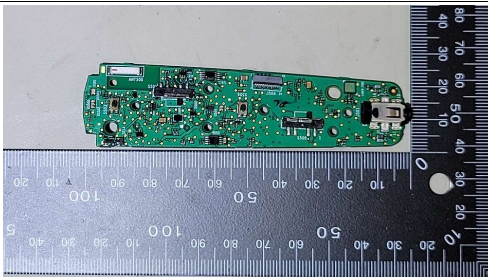
Control module, Bluetooth board – Top
