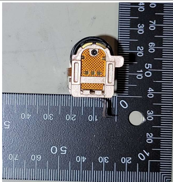
Control Module, volume wheels – Left
