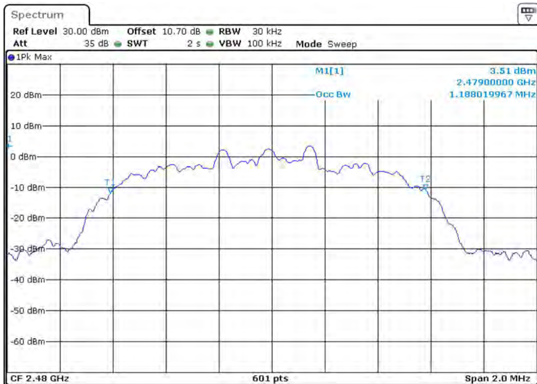
3-DH5, Tx on 2480 MHz
