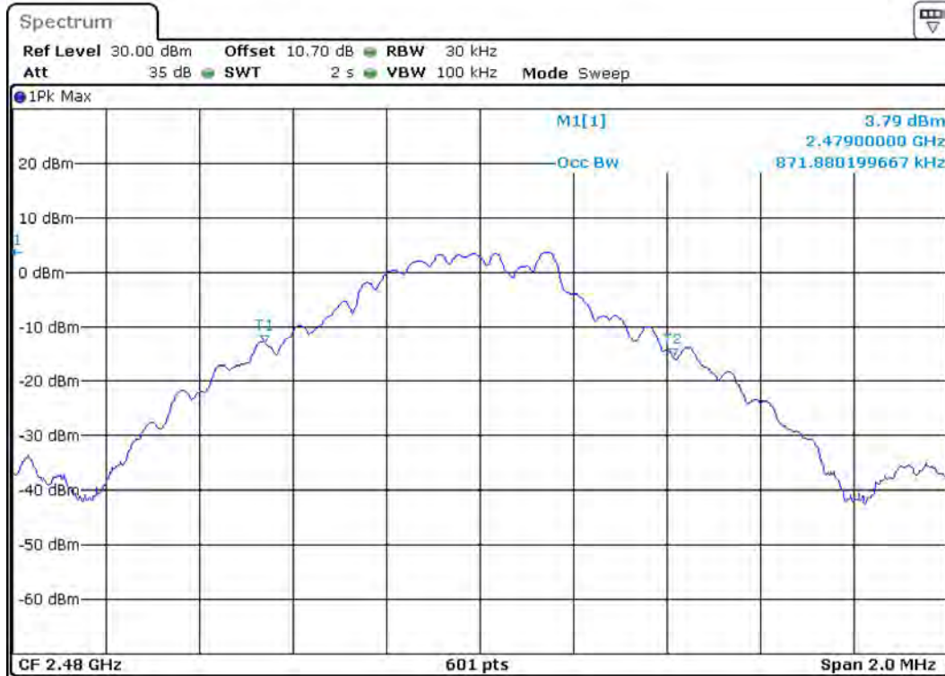
DH5, Tx on 2480 MHz
