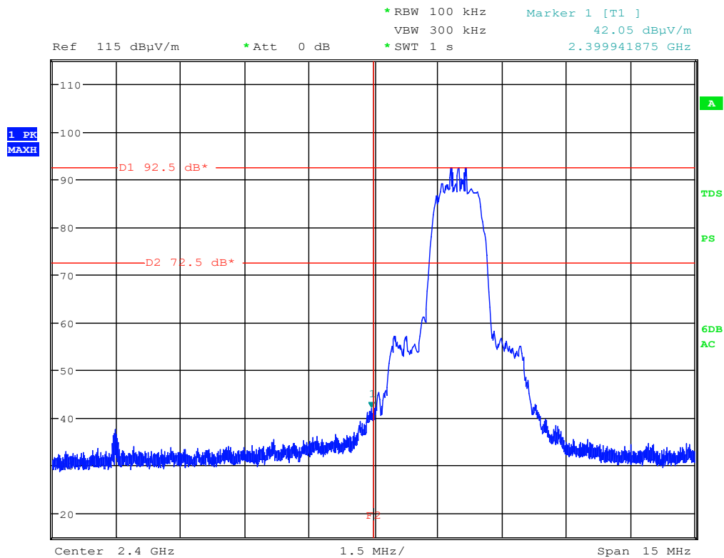
3DH5 lower and upper bandedge, hopping disabled
