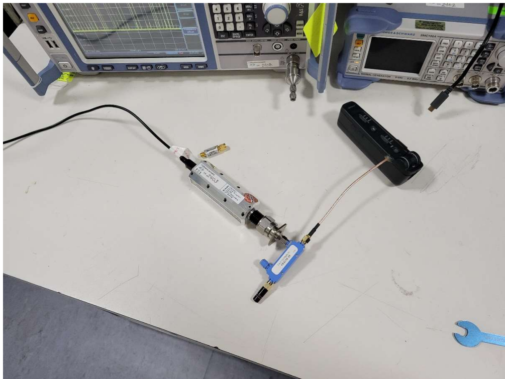
SAR Exclusion Testing
