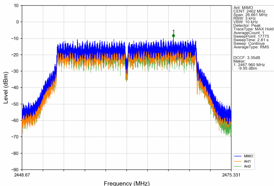
802.11ax(HEW20)_HCH_2462MHz_SU_/_MIMO_NTNV
