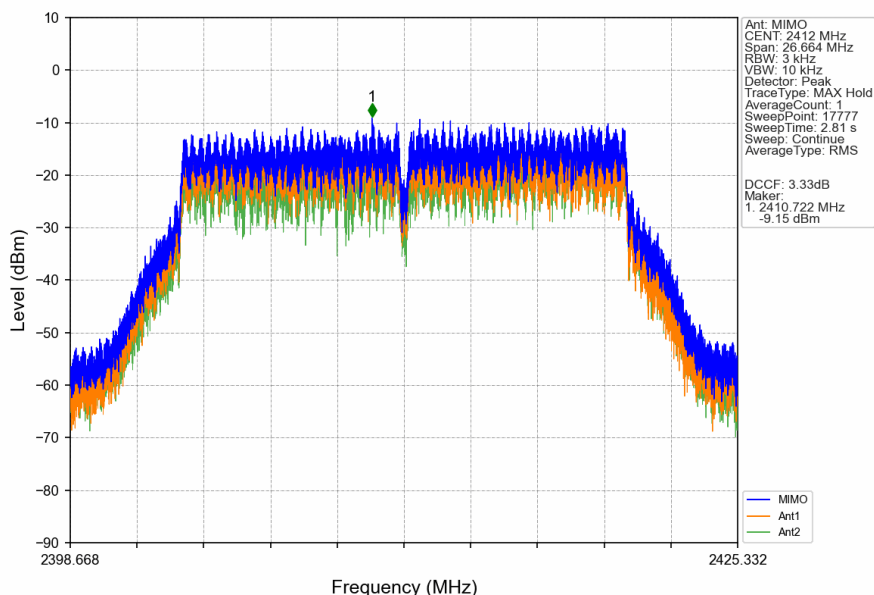
802.11ax(HEW20)_LCH_2412MHz_SU_/_MIMO_NTNV
