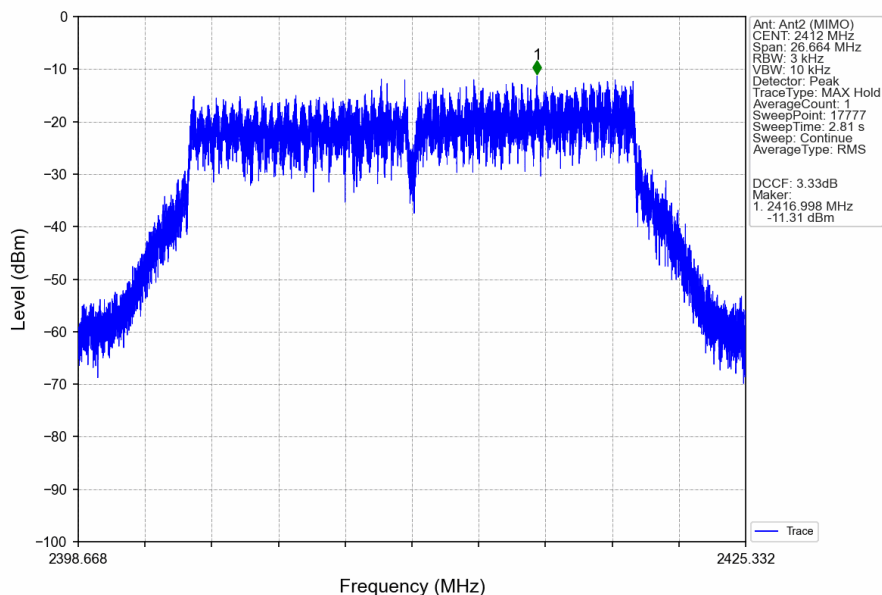
802.11ax(HEW20)_LCH_2412MHz_SU_/_MIMO_NTNV
