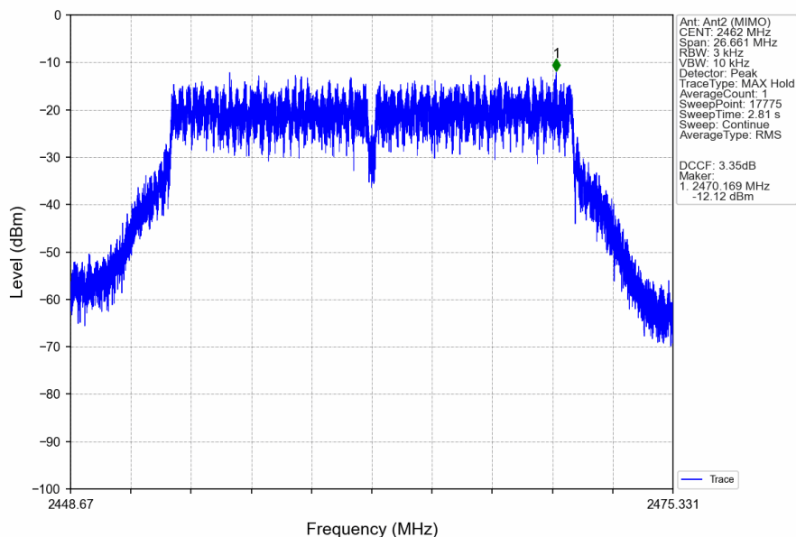
802.11ax(HEW20)_HCH_2462MHz_SU_/_MIMO_NTNV
