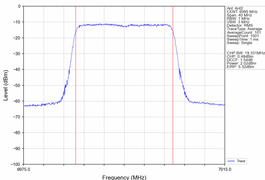
802.11ax(HEW20)_MCH_6995MHz_RU242_Left_Ant2_NTNV
