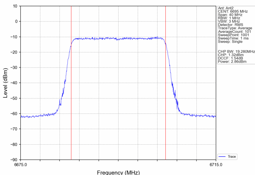
802.11ax(HEW20)_MCH_6695MHz_RU242_Left_Ant2_NTNV
