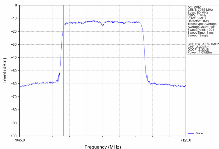
802.11ax(HEW40)_HCH_7085MHz_RU484_Left_Ant2_NTNV
