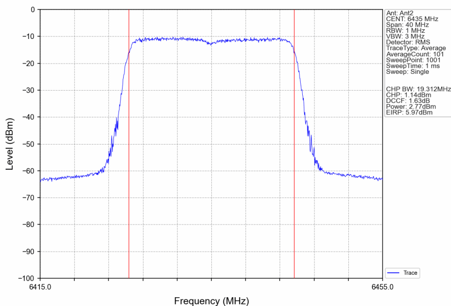
802.11ax(HEW20)_LCH_6435MHz_RU242_Left_Ant2_NTNV
