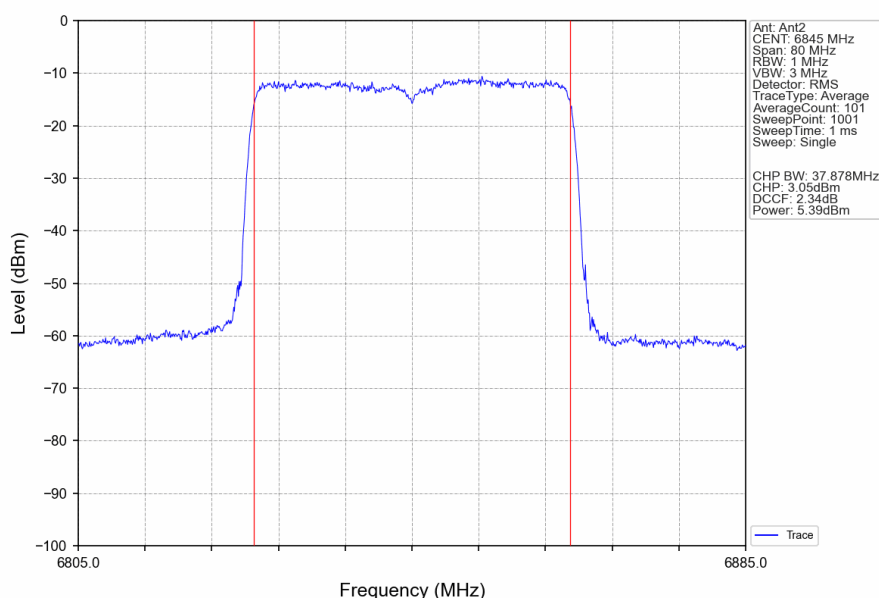
802.11ax(HEW40)_HCH_6845MHz_RU484_Left_Ant2_NTNV
