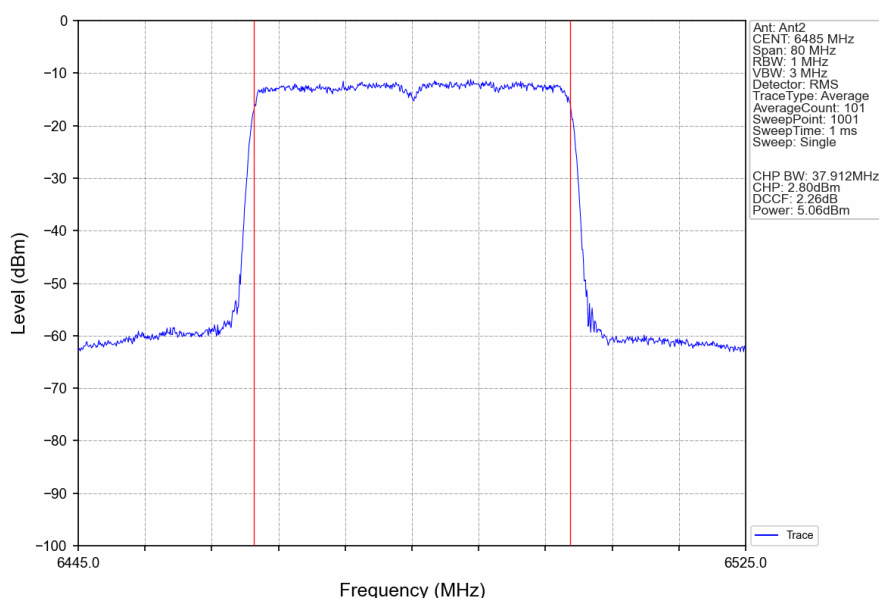
802.11ax(HEW40)_MCH_6485MHz_RU484_Left_Ant2_NTNV
