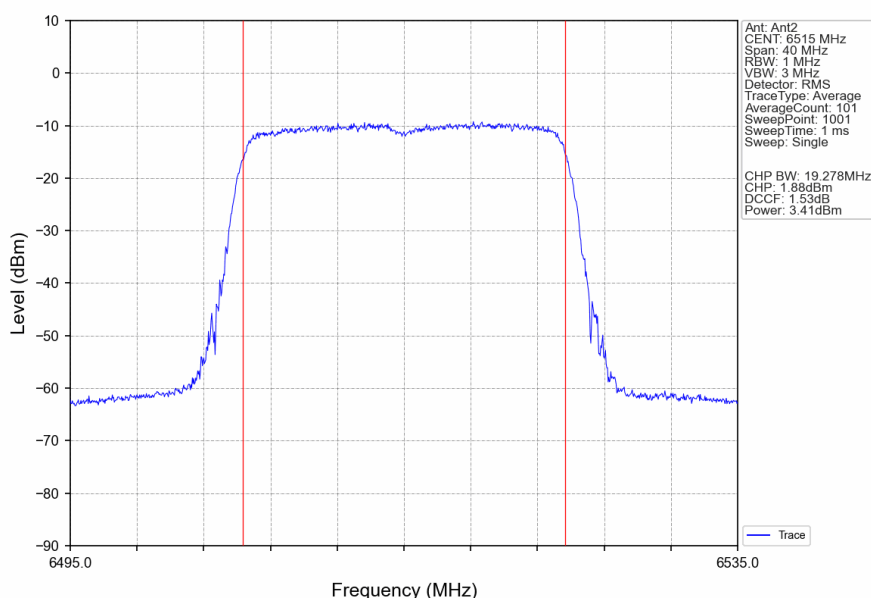
802.11ax(HEW20)_HCH_6515MHz_RU242_Left_Ant2_NTNV
