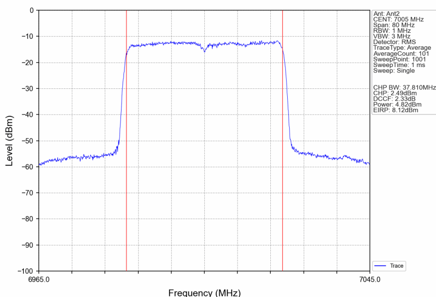
802.11ax(HEW40)_MCH_7005MHz_RU484_Left_Ant2_NTNV
