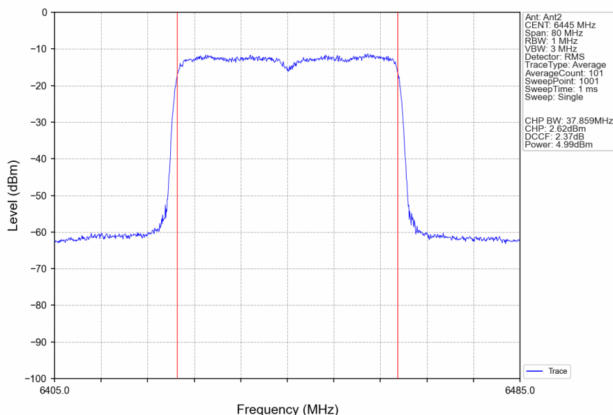
802.11ax(HEW40)_LCH_6445MHz_RU484_Left_Ant2_NTNV
