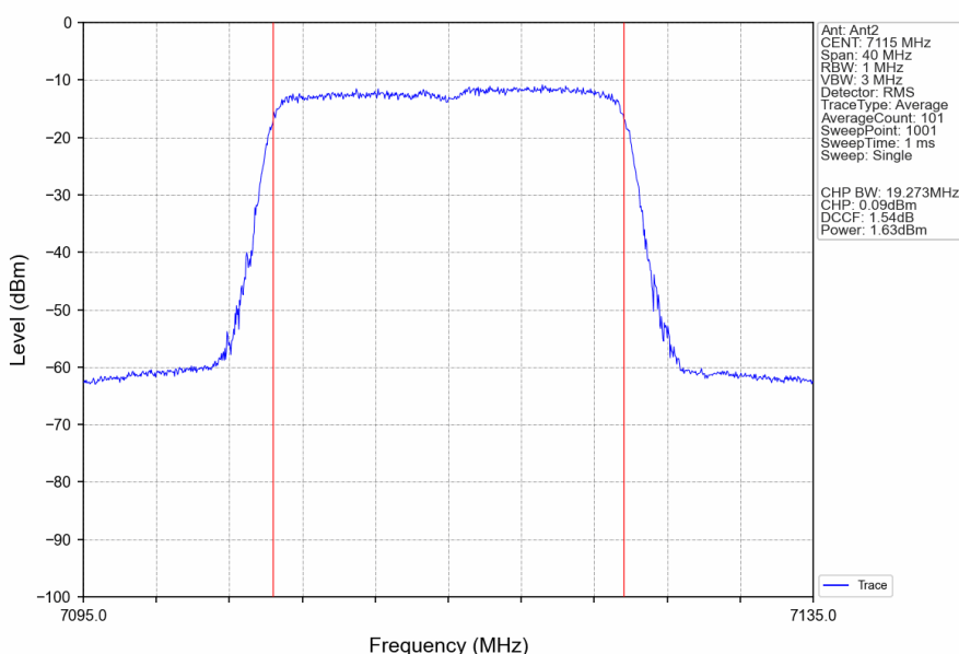
802.11ax(HEW20)_HCH_7115MHz_RU242_Left_Ant2_NTNV
