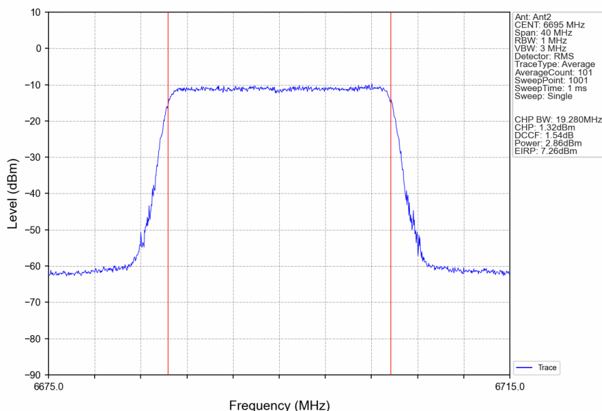
802.11ax(HEW20)_MCH_6695MHz_RU242_Left_Ant2_NTNV
