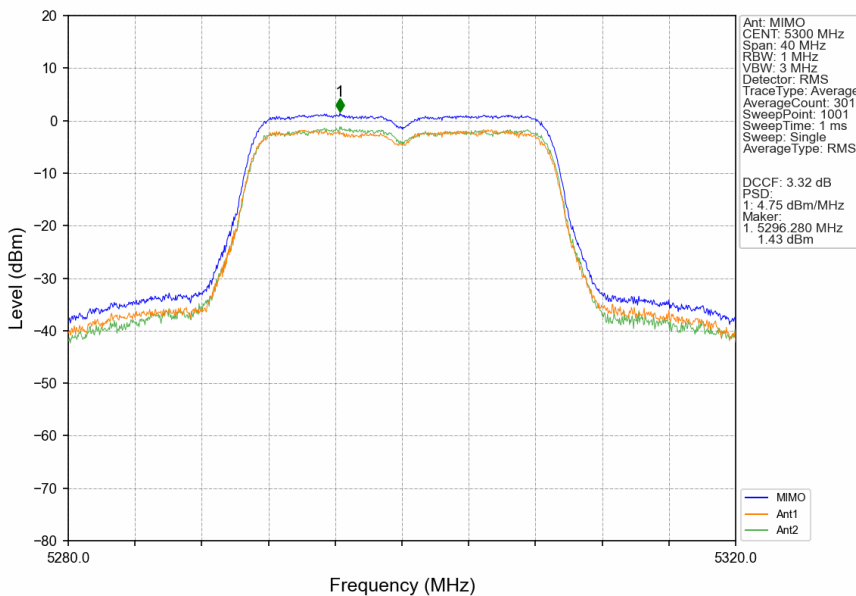
802.11ac(VHT20)_MCH_5300MHz_MIMO_NTNV
