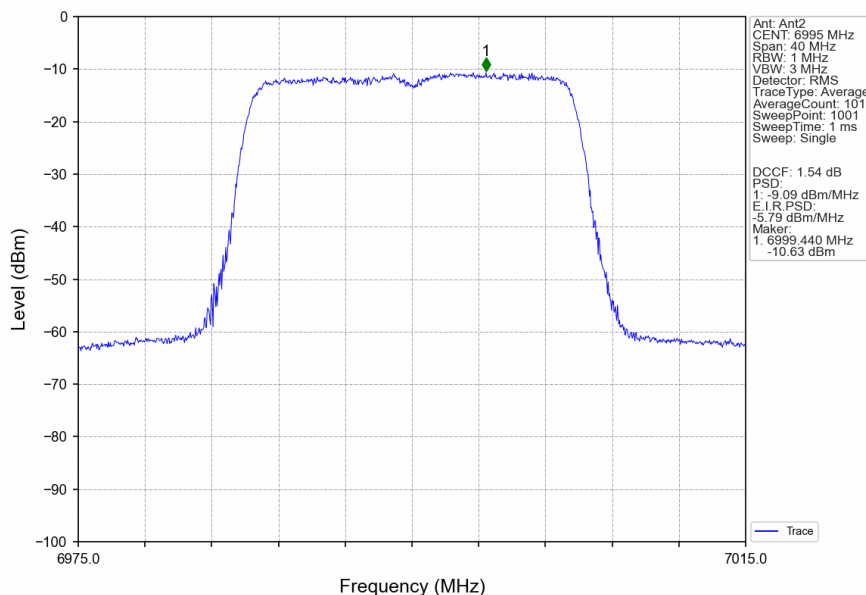
802.11ax(HEW20)_MCH_6995MHz_RU242_Left_MIMO_NTNV
