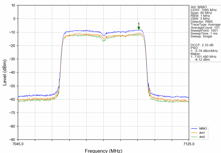
802.11ax(HEW40)_HCH_7085MHz_RU484_Left_MIMO_NTNV
