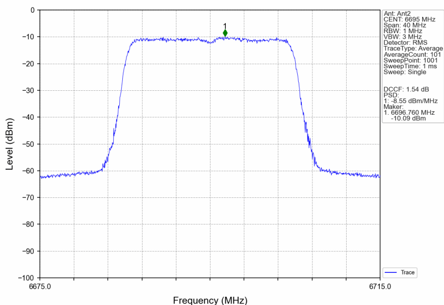
802.11ax(HEW20)_MCH_6695MHz_RU242_Left_MIMO_NTNV
