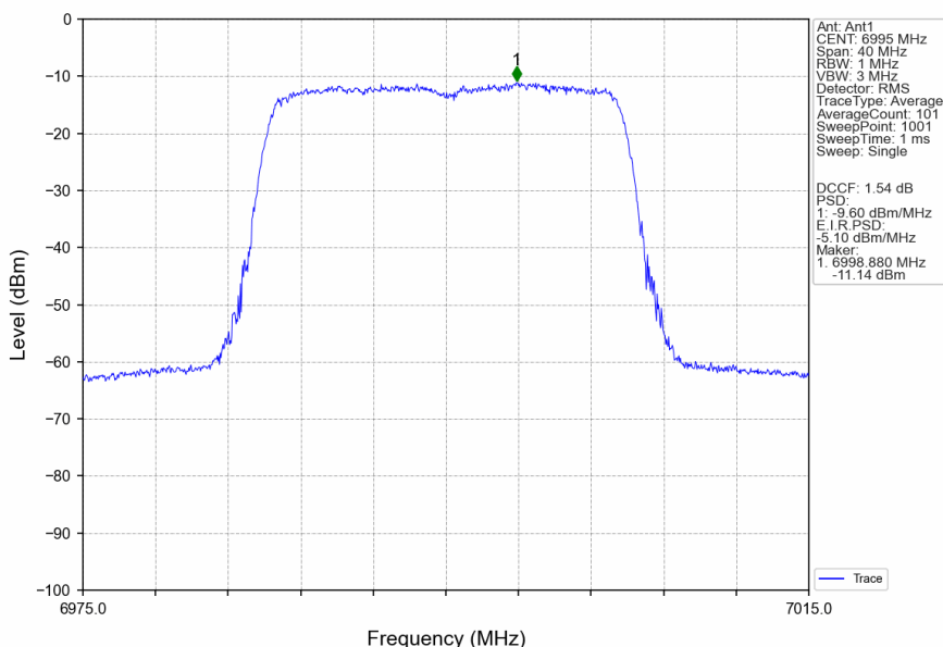
802.11ax(HEW20)_MCH_6995MHz_RU242_Left_Ant1_NTNV
