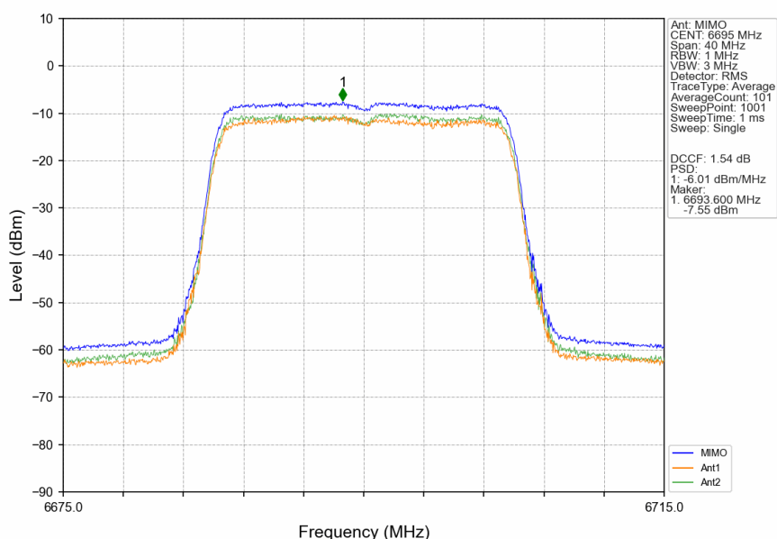
802.11ax(HEW20)_MCH_6695MHz_RU242_Left_MIMO_NTNV
