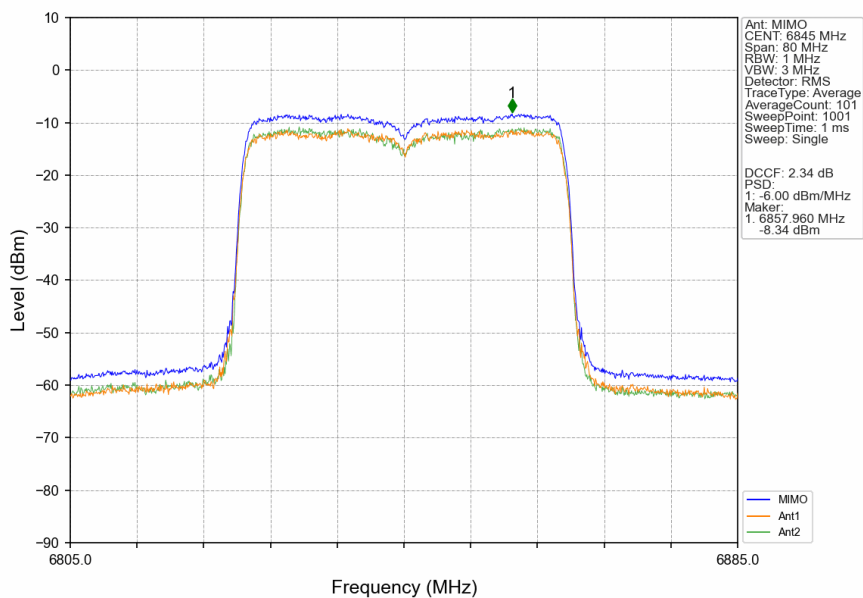
802.11ax(HEW40)_HCH_6845MHz_RU484_Left_MIMO_NTNV
