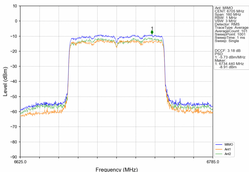
802.11ax(HEW80)_MCH_6705MHz_RU996_Left_MIMO_NTNV
