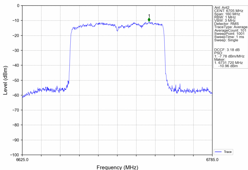
802.11ax(HEW80)_MCH_6705MHz_RU996_Left_MIMO_NTNV
