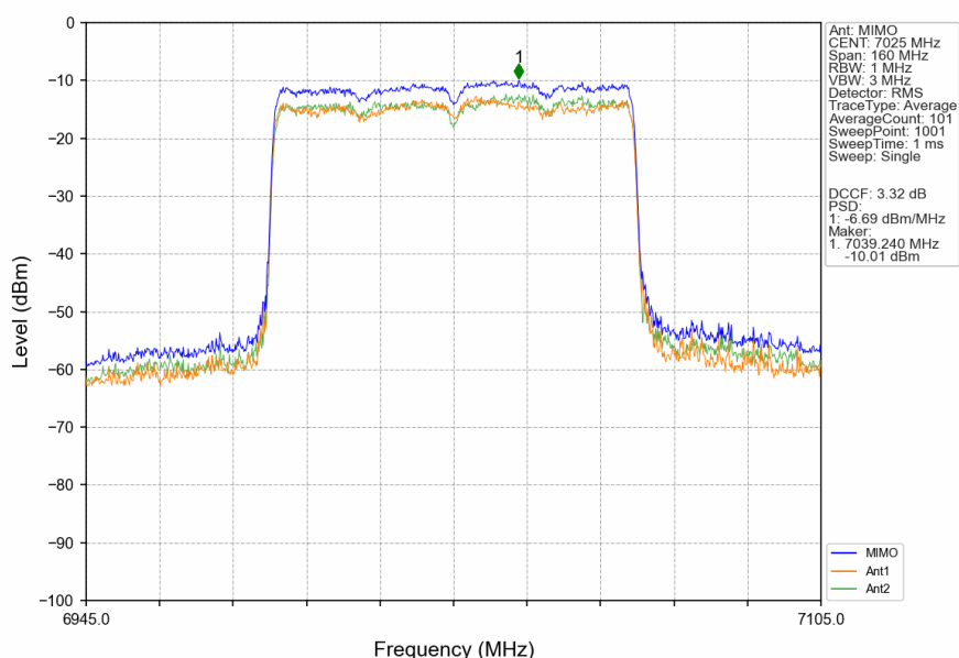
802.11ax(HEW80)_HCH_7025MHz_RU996_Left_MIMO_NTNV
