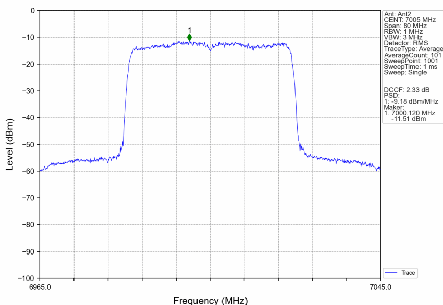
802.11ax(HEW40)_MCH_7005MHz_RU484_Left_Ant2_NTNV
