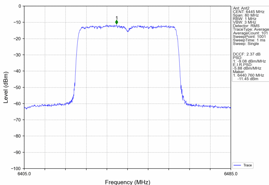
802.11ax(HEW40)_LCH_6445MHz_RU484_Left_MIMO_NTNV
