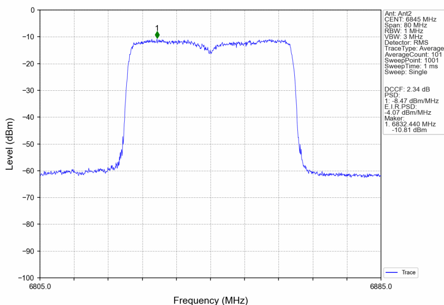
802.11ax(HEW40)_HCH_6845MHz_RU484_Left_MIMO_NTNV
