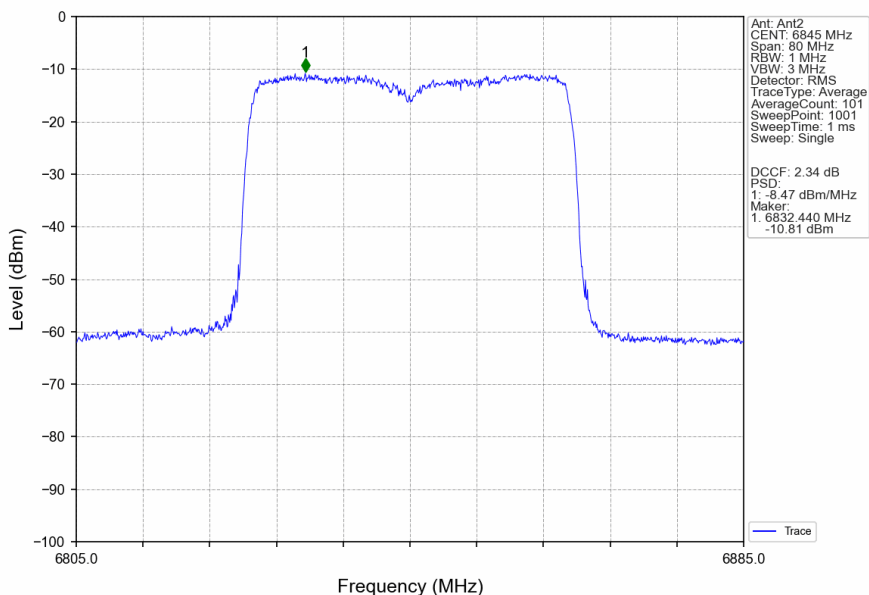
802.11ax(HEW40)_HCH_6845MHz_RU484_Left_MIMO_NTNV
