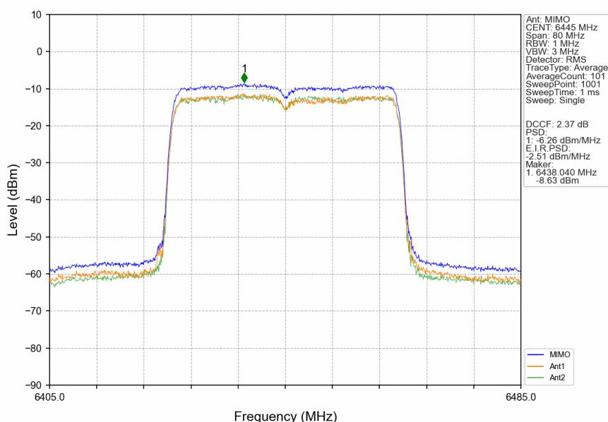
802.11ax(HEW40)_LCH_6445MHz_RU484_Left_MIMO_NTNV
