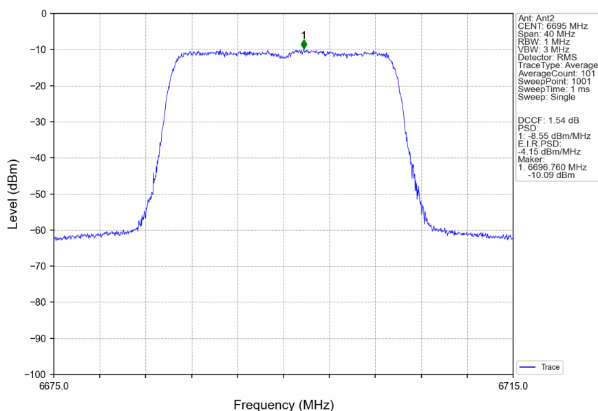
802.11ax(HEW20)_MCH_6695MHz_RU242_Left_MIMO_NTNV
