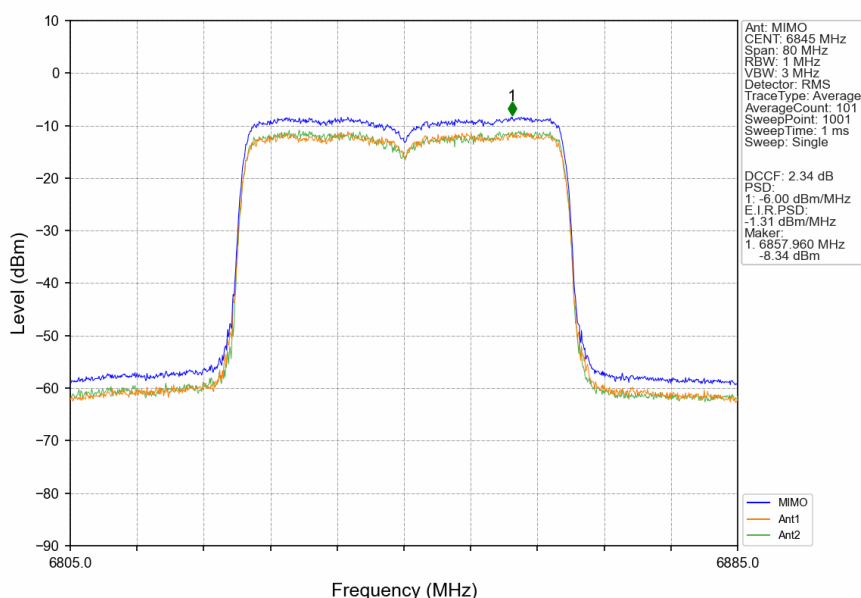
802.11ax(HEW40)_HCH_6845MHz_RU484_Left_MIMO_NTNV
