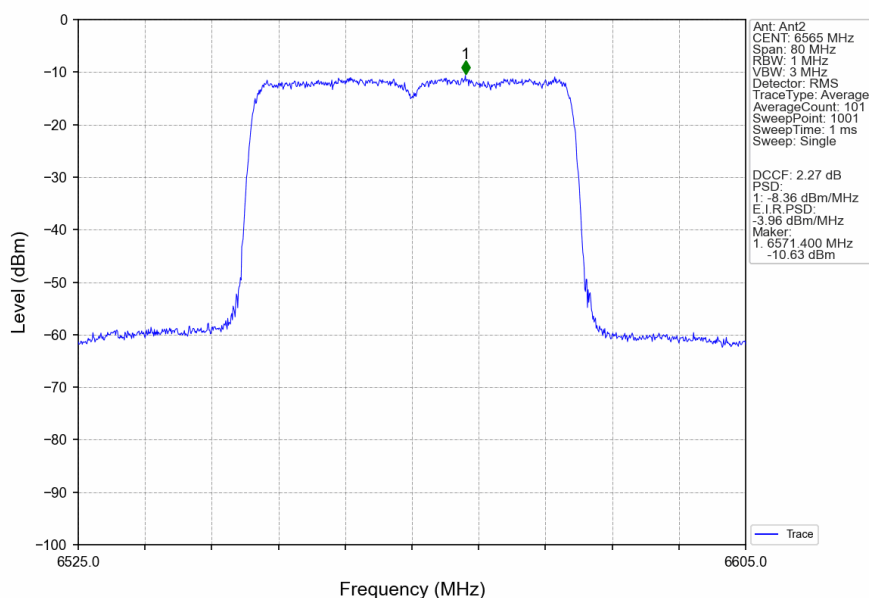
802.11ax(HEW40)_LCH_6565MHz_RU484_Left_MIMO_NTNV
