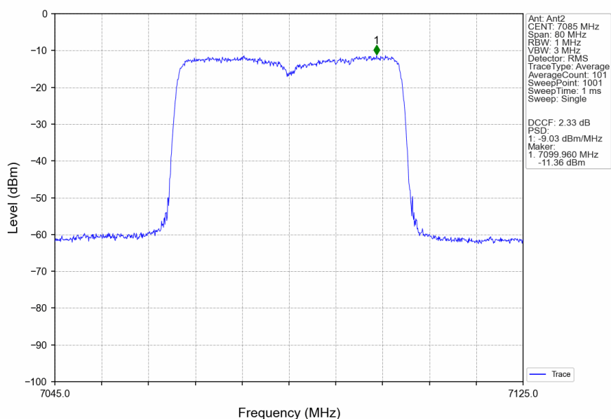
802.11ax(HEW40)_HCH_7085MHz_RU484_Left_MIMO_NTNV
