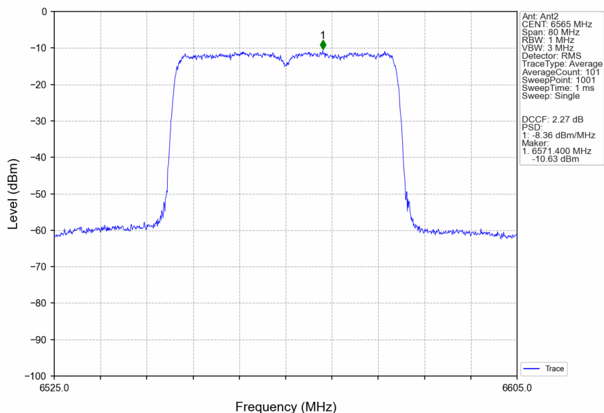
802.11ax(HEW40)_LCH_6565MHz_RU484_Left_MIMO_NTNV
