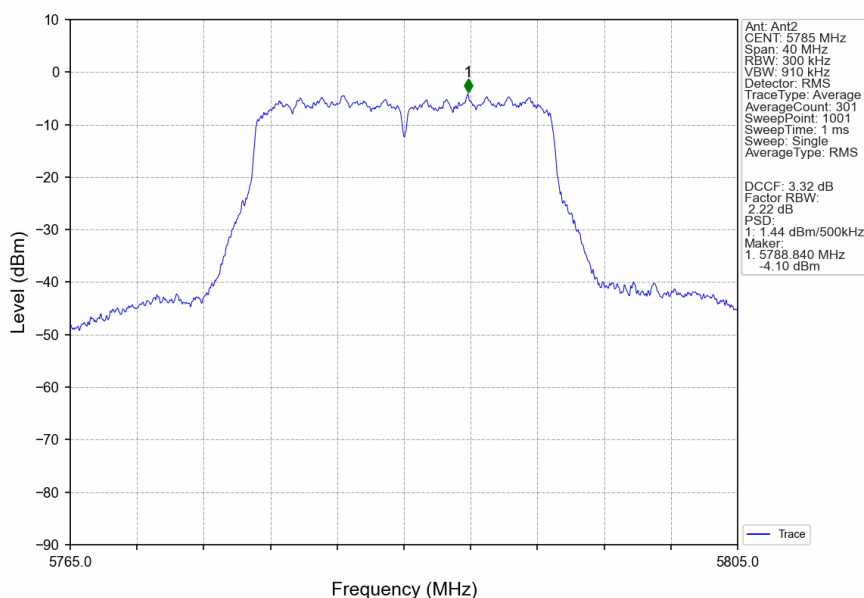
802.11ac(VHT20)_MCH_5785MHz_MIMO_NTNV
