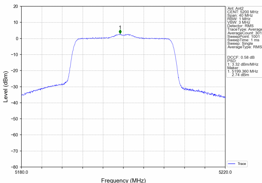
802.11ax(HEW20)_MCH_5200MHz_SU_/_Ant2_NTNV
