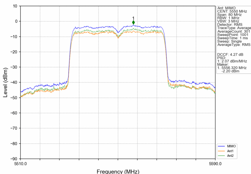
802.11ax(HEW40)_MCH_5550MHz_SU_/_MIMO_NTNV
