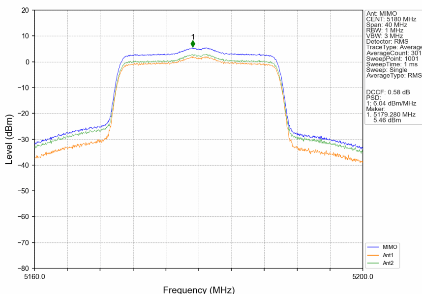
802.11ax(HEW20)_LCH_5180MHz_SU_ / _MIMO_NTNV
