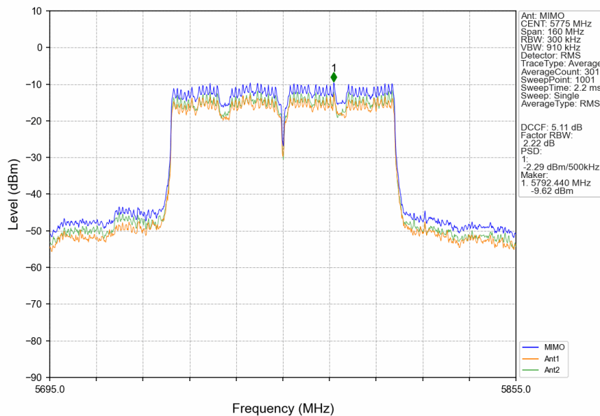
802.11ac(VHT80)_MCH_5775MHz_MIMO_NTNV
