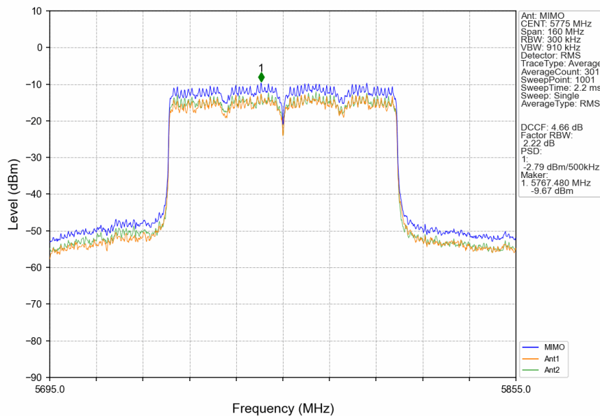
802.11ax(HEW80)_MCH_5775MHz_SU_/_MIMO_NTNV
