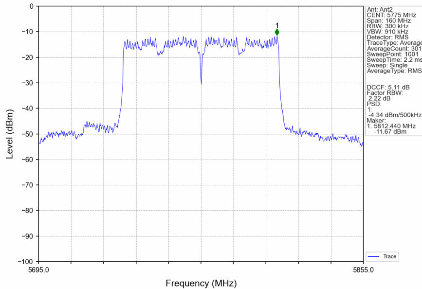
802.11ac(VHT80)_MCH_5775MHz_MIMO_NTNV
