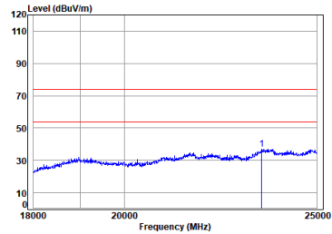
BLE_2M_TX_CH_00_Vertical
