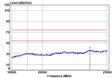
BLE_1M_TX_CH_00_Vertical
