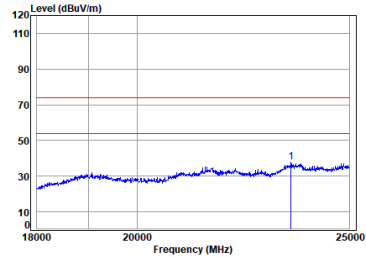
BLE_1M_TX_CH_39_Vertical
