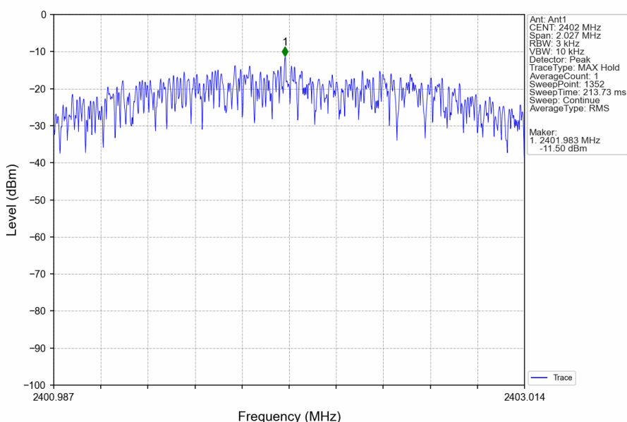
2M_LCH_2402MHz_Ant1_NTNV
