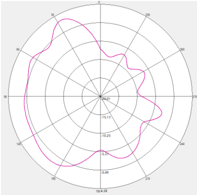
6550MHZ V-pol
