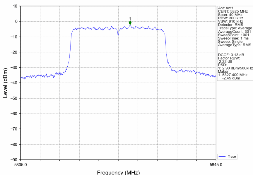
802.11ax(HEW20)_HCH_5825MHz_RU242_Left_Ant1_NTNV
