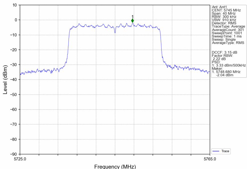
802.11ax(HEW20)_LCH_5745MHz_RU242_Left_Ant1_NTNV
