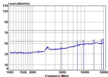
BT_DH5_TX_CH_00_Vertical
