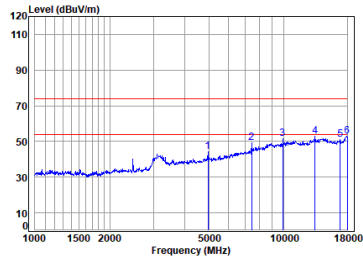
BT_DH5_TX_CH_78_Horizontal
