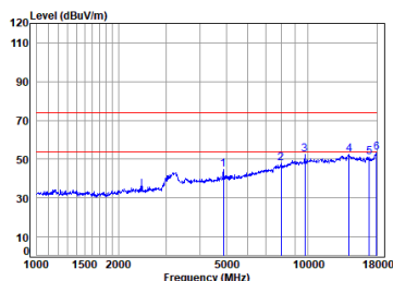
BT_DH5_TX_CH_39_Vertical
