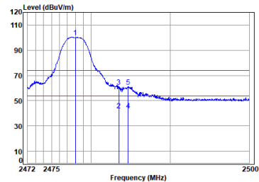
QHS_6M_TX_CH_38_Vertical
