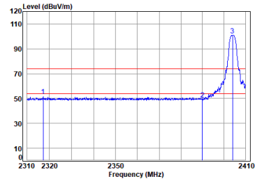
QHS_6M_TX_CH_01_Vertical
