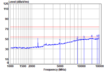
QHS_6M_TX_CH_19_Vertical
