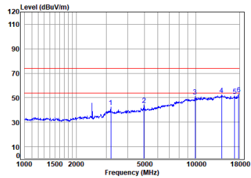
QHS_6M_TX_CH_01_Vertical
