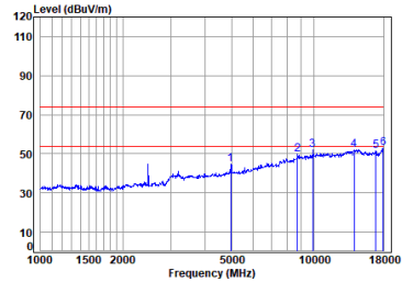
QHS_6M_TX_CH_38_Vertical
