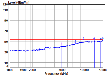
QHS_6M_TX_CH_38_Horizontal
