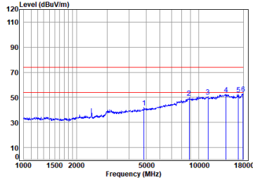
QHS_6M_TX_CH_19_Horizontal
