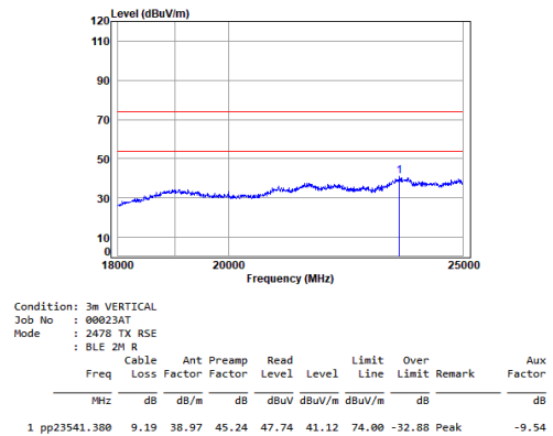
BLE_2M_TX_CH_38_Vertical
