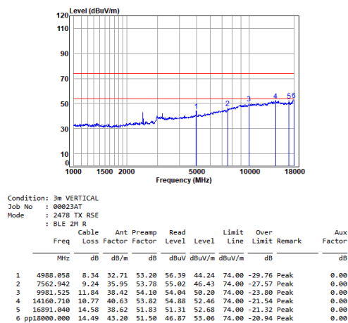
BLE_2M_TX_CH_38_Vertical
