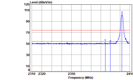
BLE_1M_TX_CH_00_Horizontal
