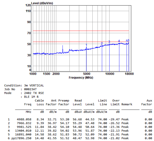
BLE_1M_TX_CH_00_Vertical
