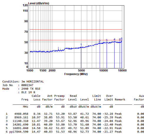
BLE_1M_TX_CH_19_Horizontal
