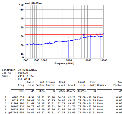
BLE_2M_TX_CH_19_Horizontal
