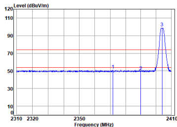
BLE_2M_TX_CH_01_Vertical
