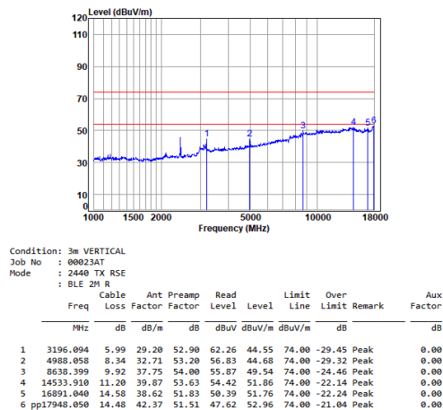
BLE_2M_TX_CH_19_Vertical
