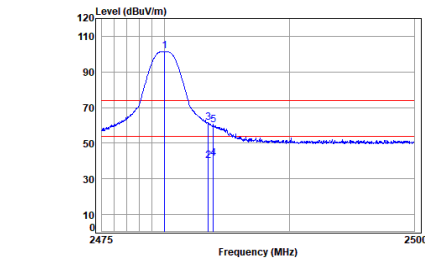
BLE_1M_TX_CH_39_Horizontal
