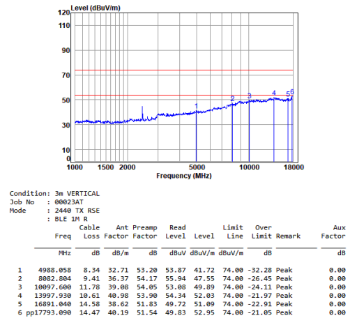
BLE_1M_TX_CH_19_Vertical
