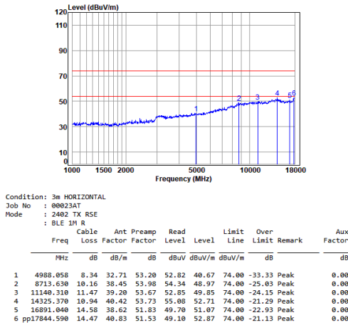
BLE_1M_TX_CH_00_Horizontal
