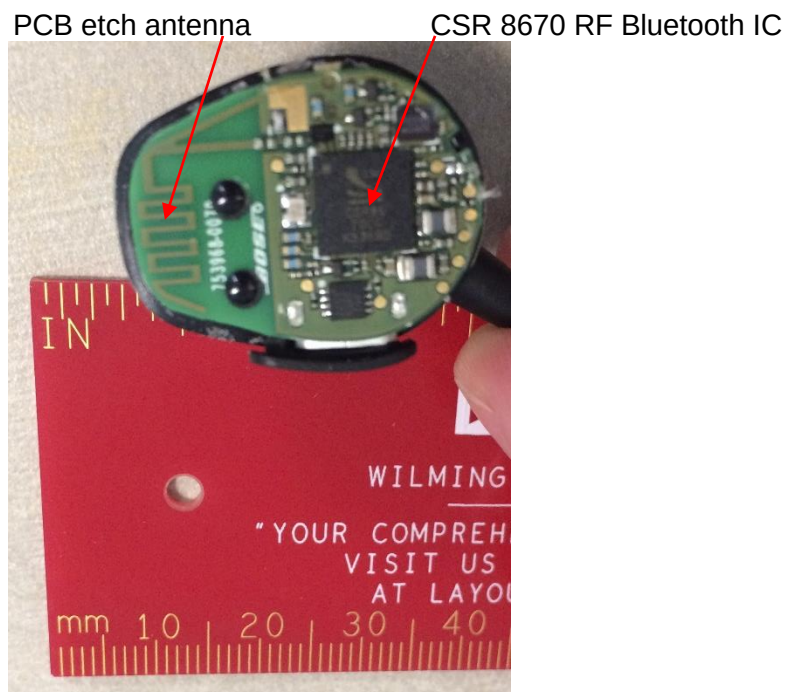
Right earbud, main PCB bottom side
