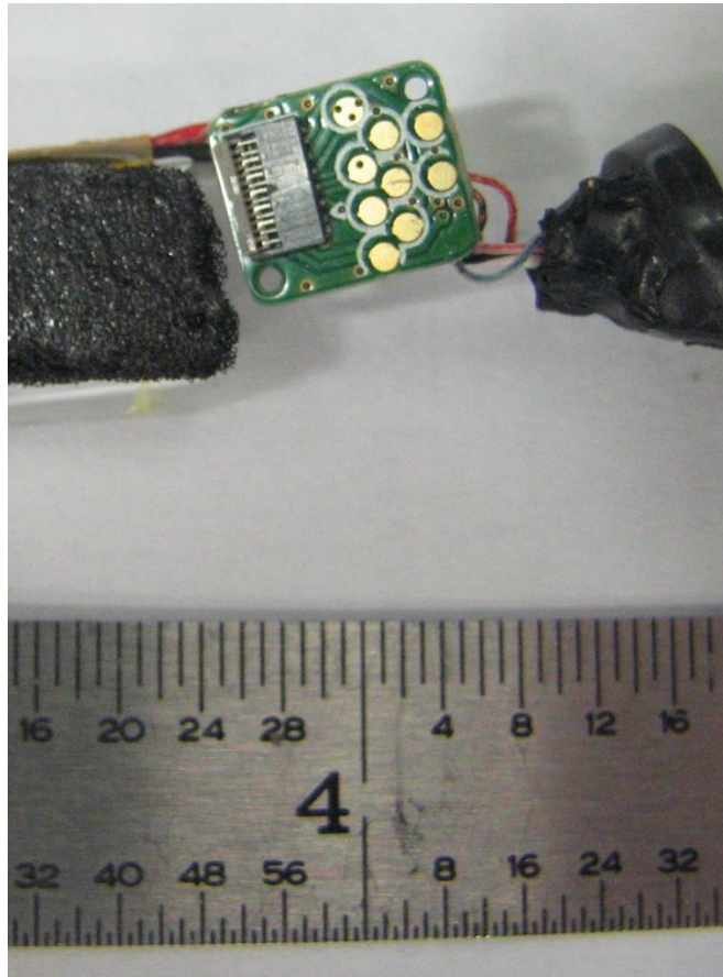
Neckband flex interface board
