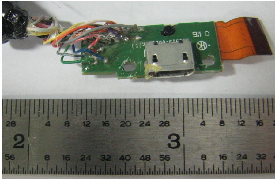
USB board
