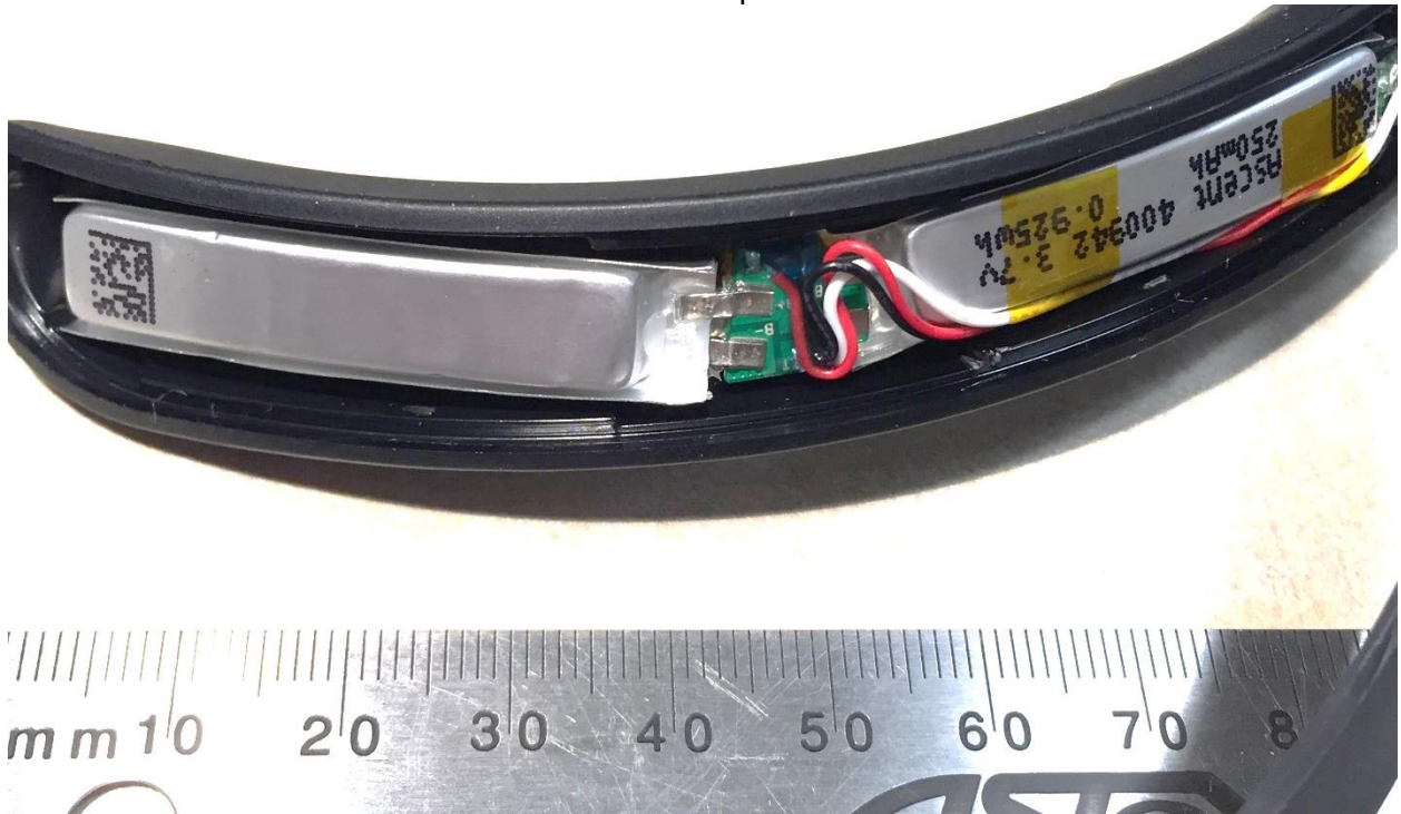
Batteries top view
