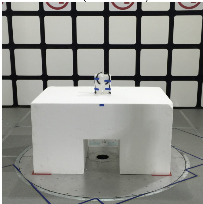
RADIATED PHOTO (BELOW 1 GHz)
