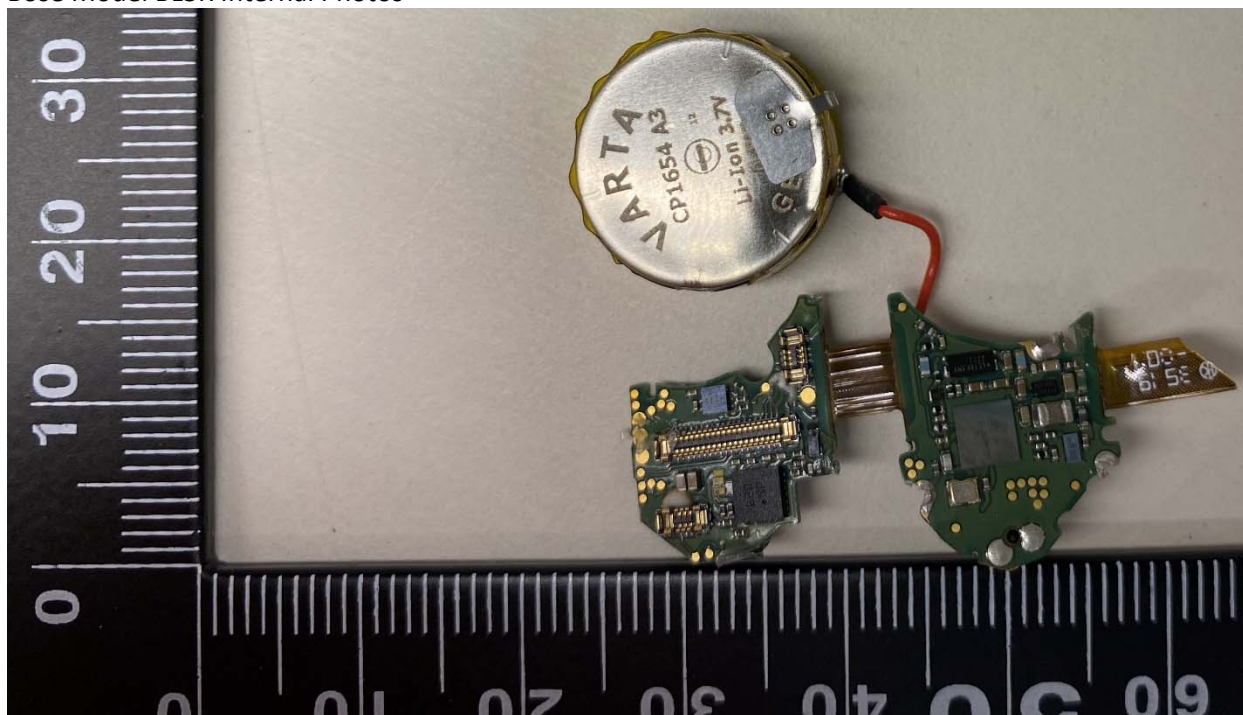
Bose Model BL3R Internal Photos
