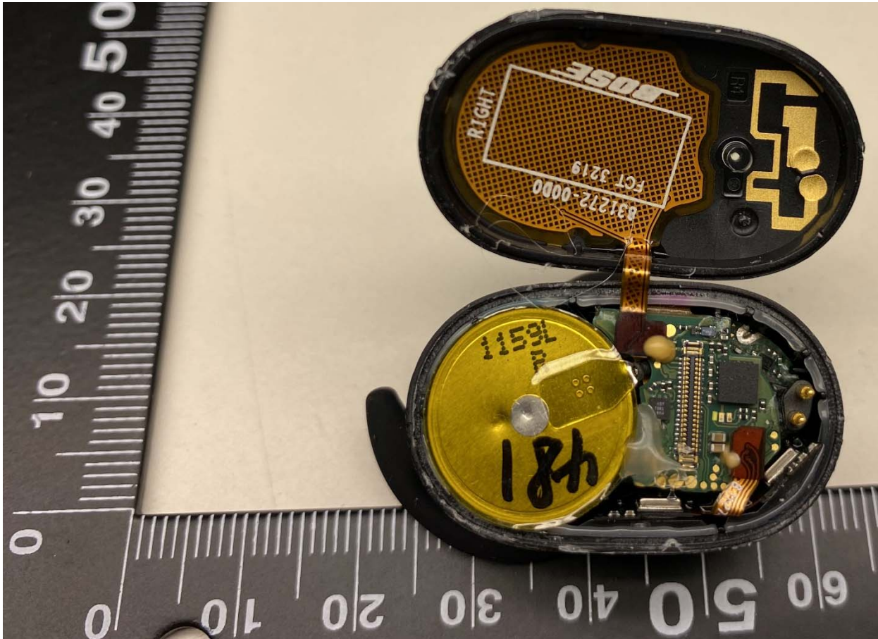
Bose Model BL3R Internal Photos
