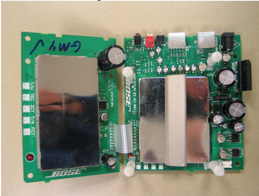
Covers removed
