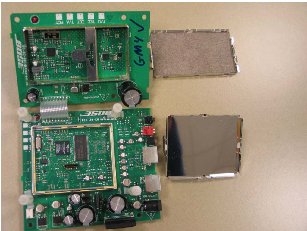
Covers removed
