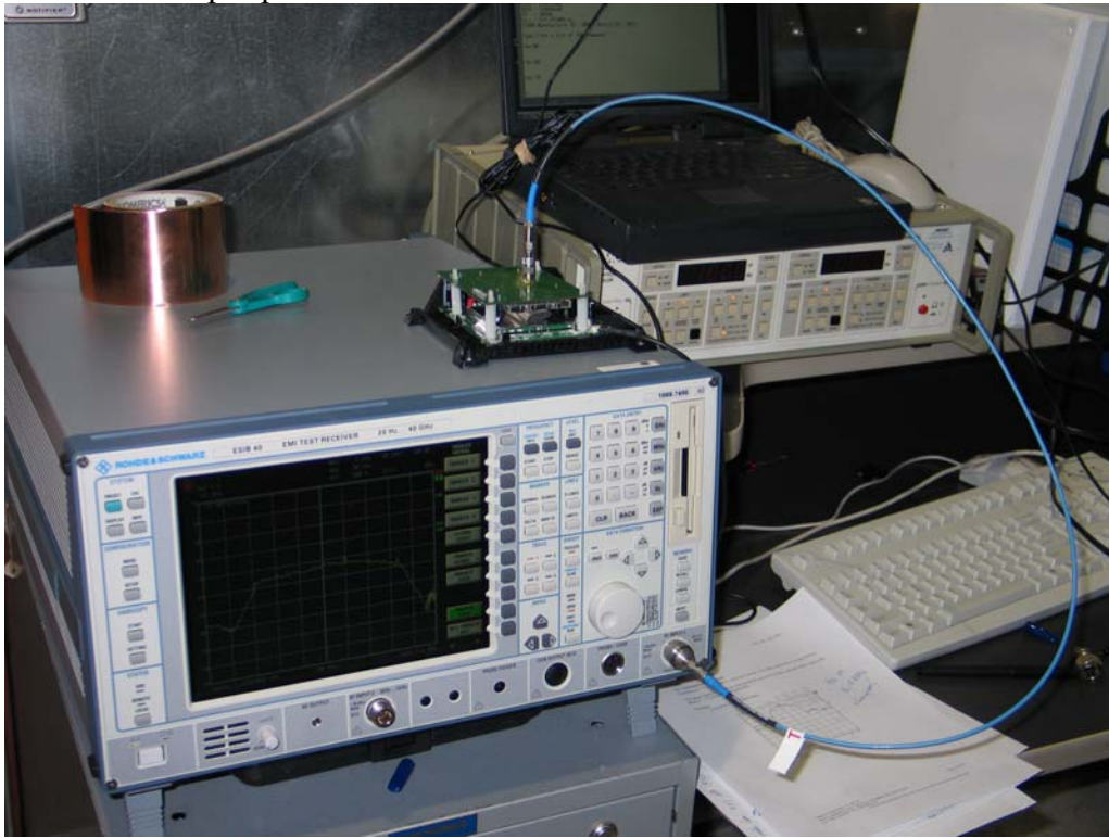
Harmonics measurement (radiated)
