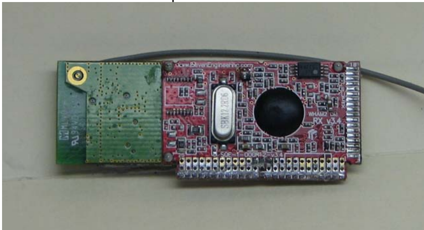
radio control module and partial backside of ML5800 radio module.
