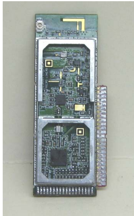
radio control module and partial backside of ML5800 radio module.
