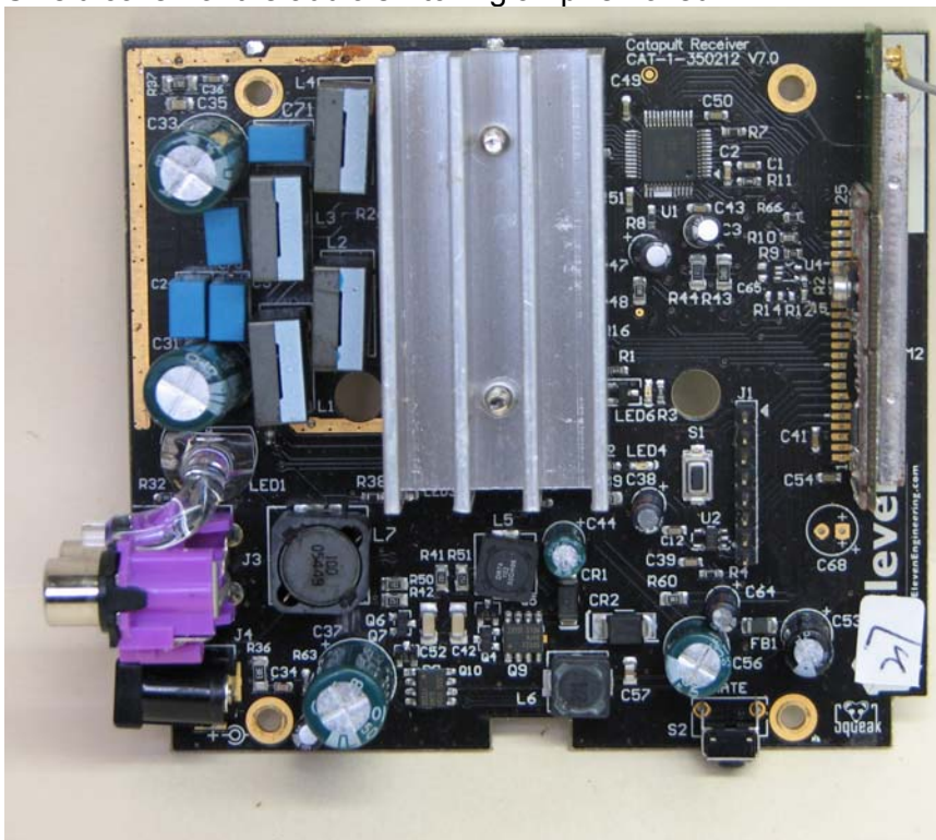
Shield cover for the audio switching amp removed
