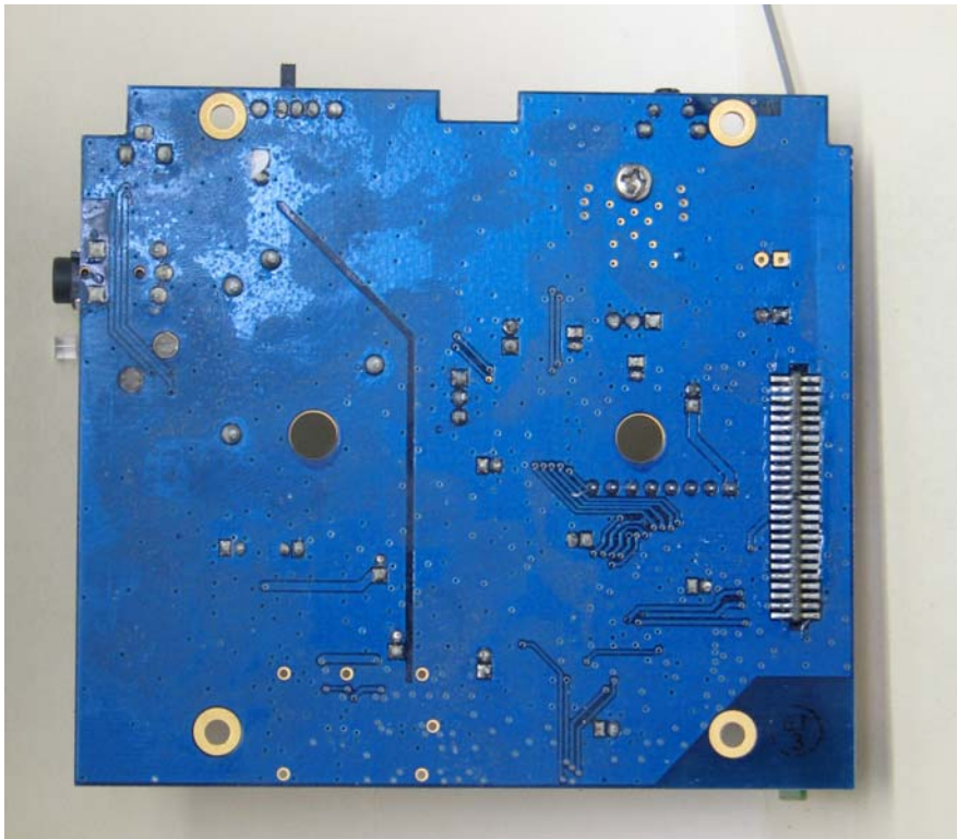
TX unit backside
