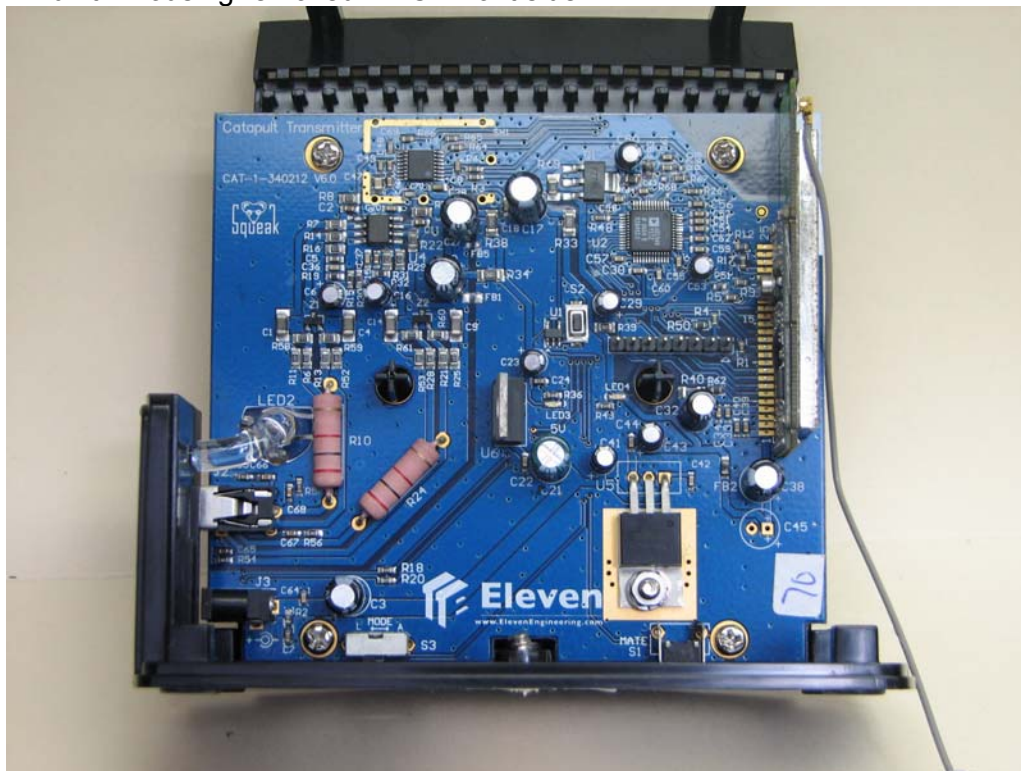
TX unit backside
