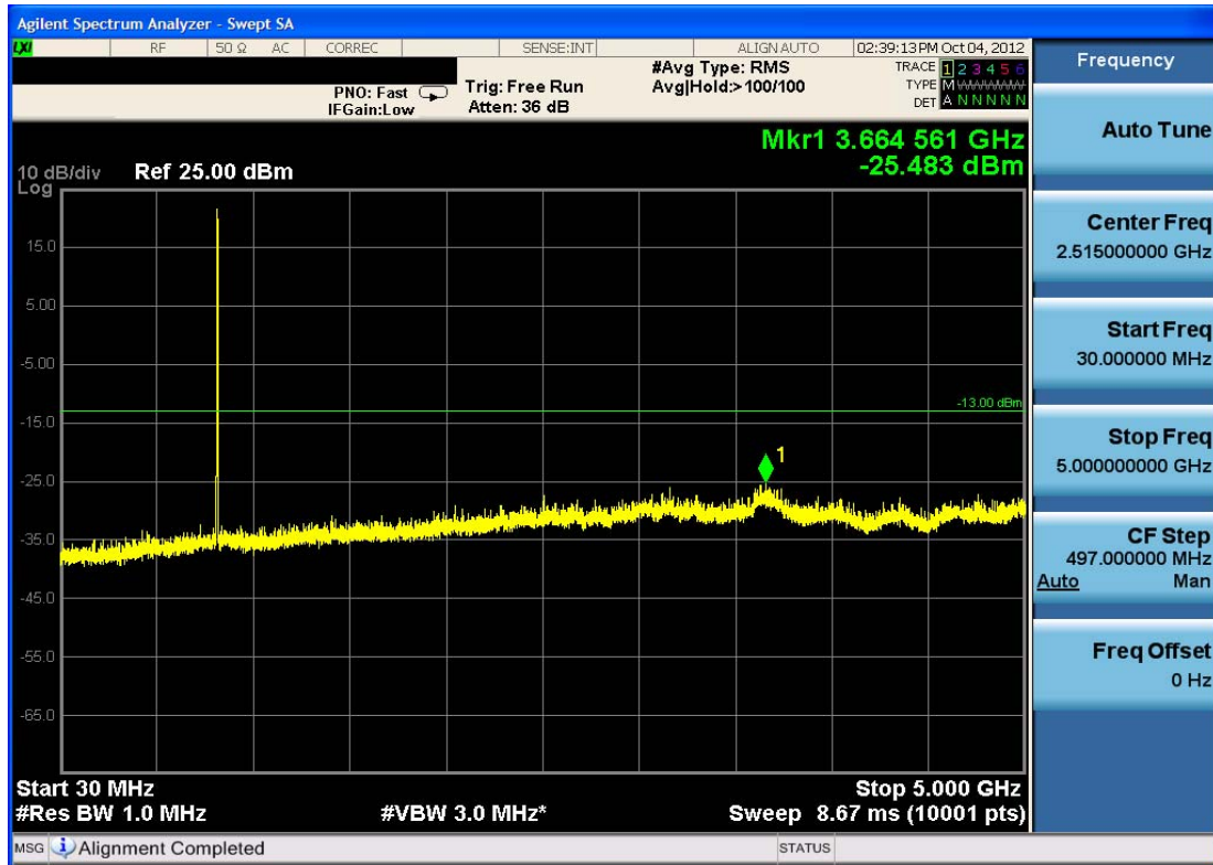
Plot 7-7. Conducted Spurious Plot (Cellular WCDMA Mode – Ch. 4183)
