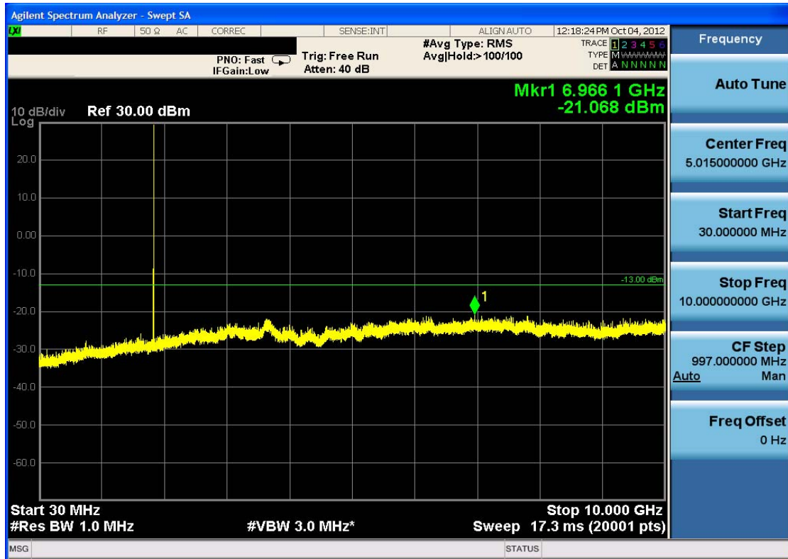
Plot 7-13. Conducted Spurious Plot (PCS GSM Mode – Ch. 512)
