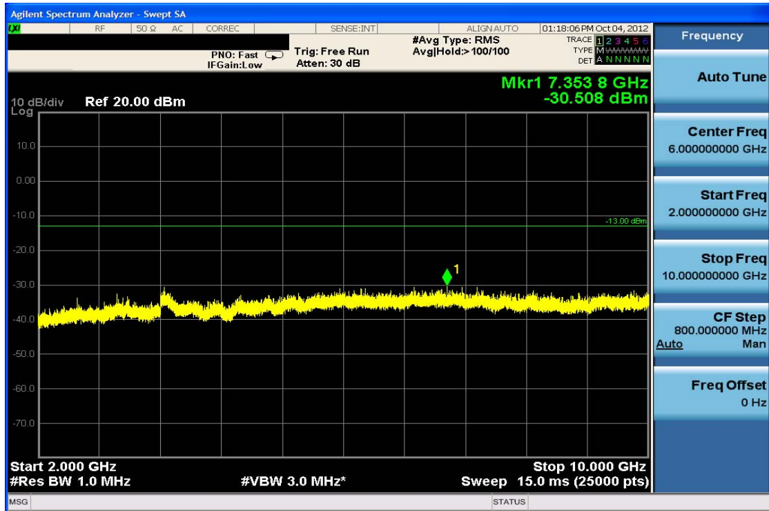
Plot 7-7. Conducted Spurious Plot (Cellular GSM Mode – Ch. 190)
