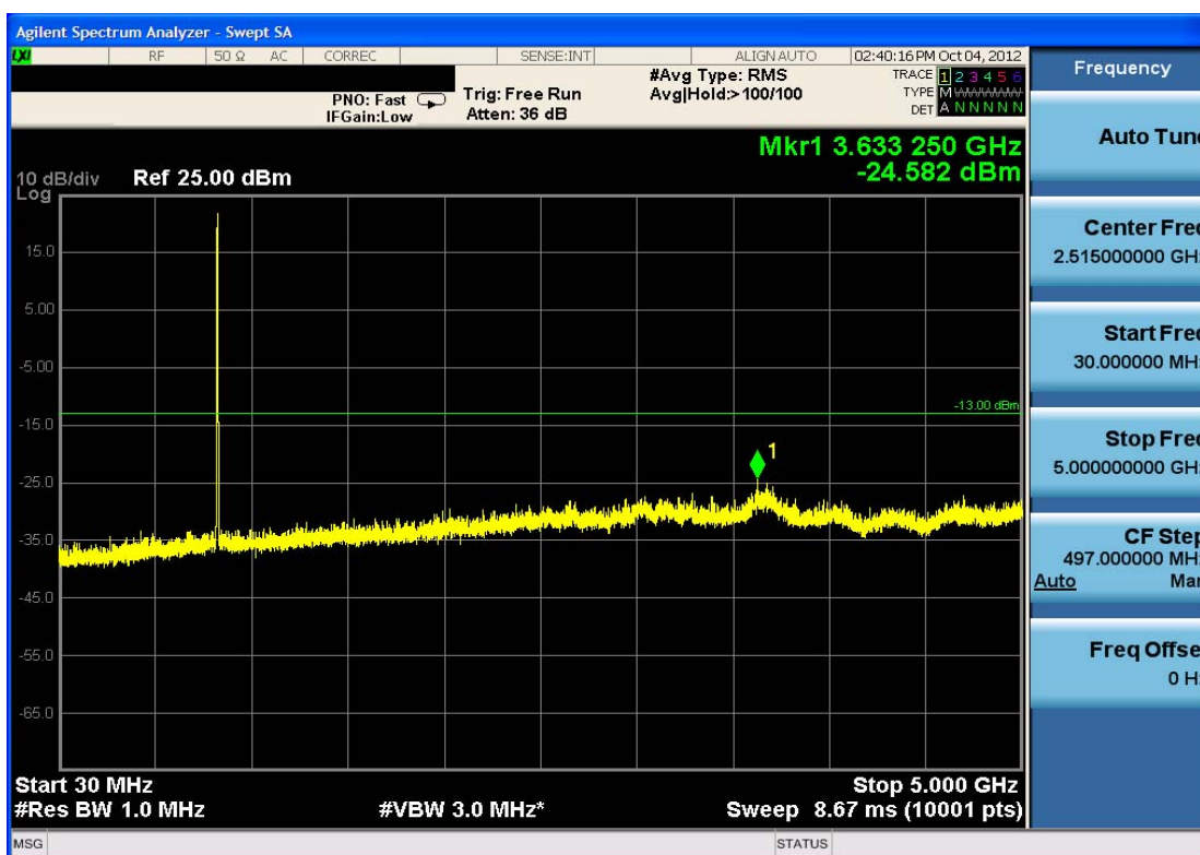
Plot 7-10. Conducted Spurious Plot (Cellular WCDMA Mode – Ch. 4233)
