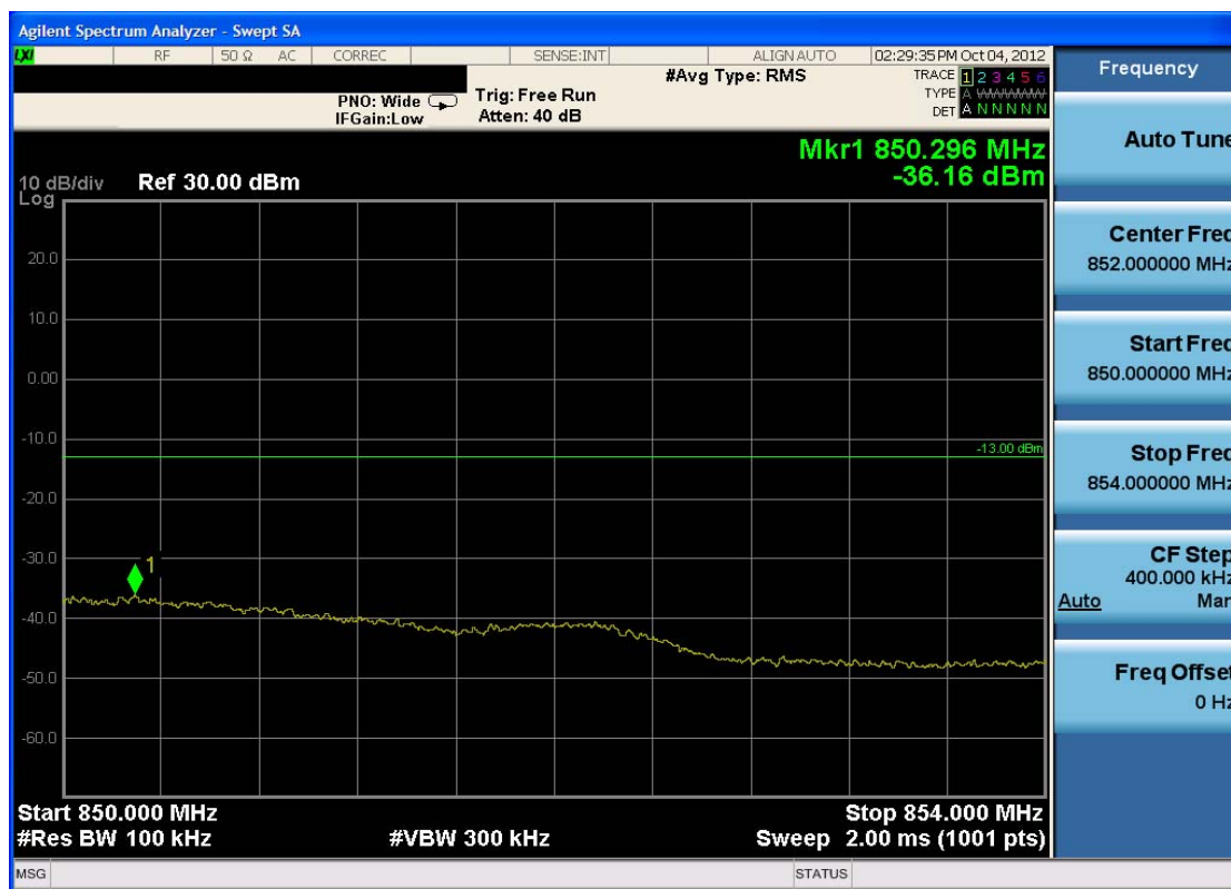
Plot 7-13. 4MHz Span Plot (Cellular WCDMA Mode – Ch. 4233)
