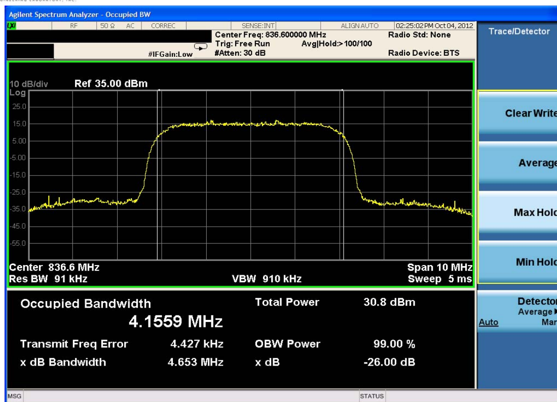
Plot 7-9. Occupied Bandwidth Plot (Cellular WCDMA Mode – Ch. 4183)
