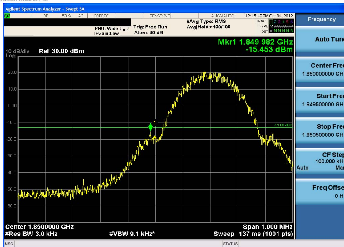
Plot 7-15. Band Edge Plot (PCS GSM Mode – Ch. 512)
