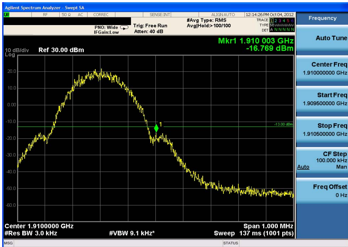
Plot 7-22. Band Edge Plot (PCS GSM Mode – Ch. 810)
