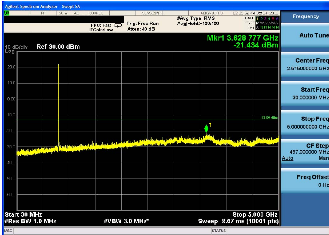
Plot 7-3. Conducted Spurious Plot (Cellular WCDMA Mode – Ch. 4132)
