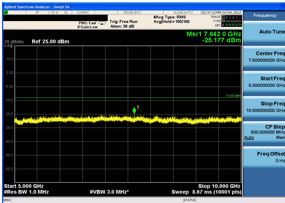
Plot 7-4. Conducted Spurious Plot (Cellular WCDMA Mode – Ch. 4132)
