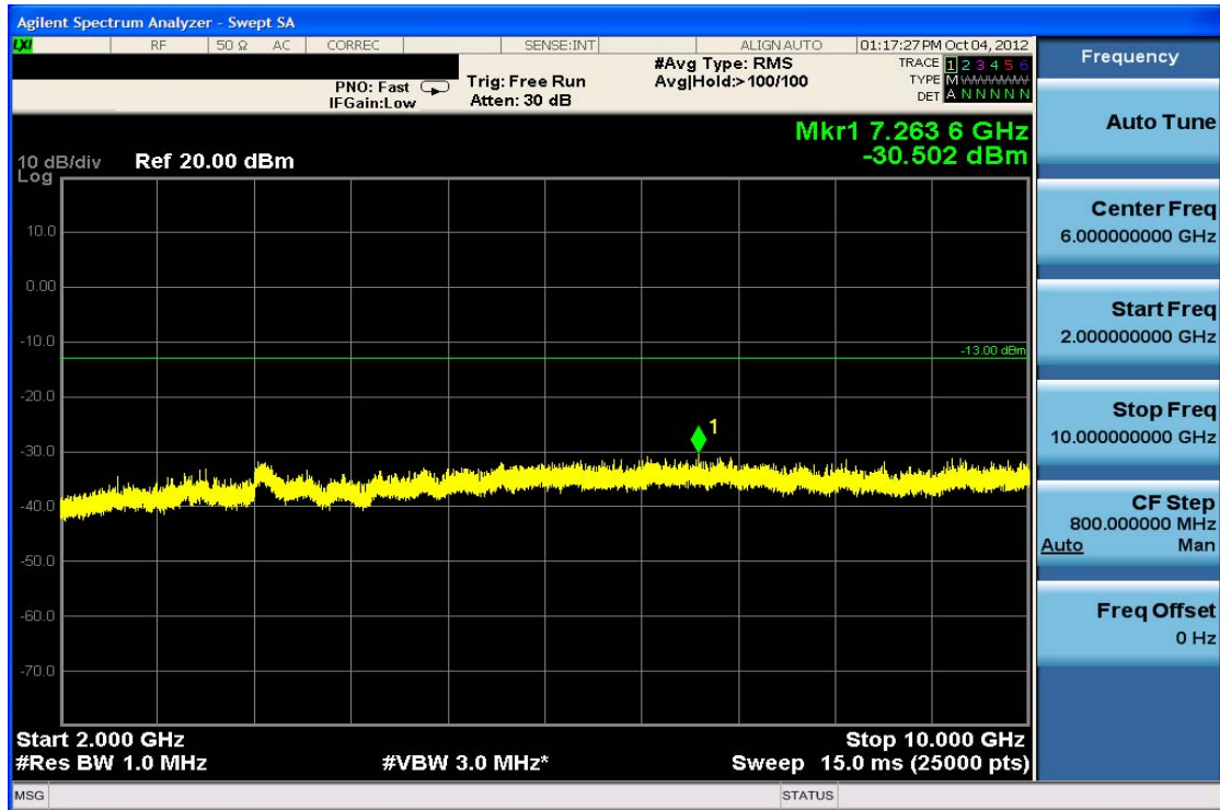
Plot 7-3. Conducted Spurious Plot (Cellular GSM Mode – Ch. 128)
