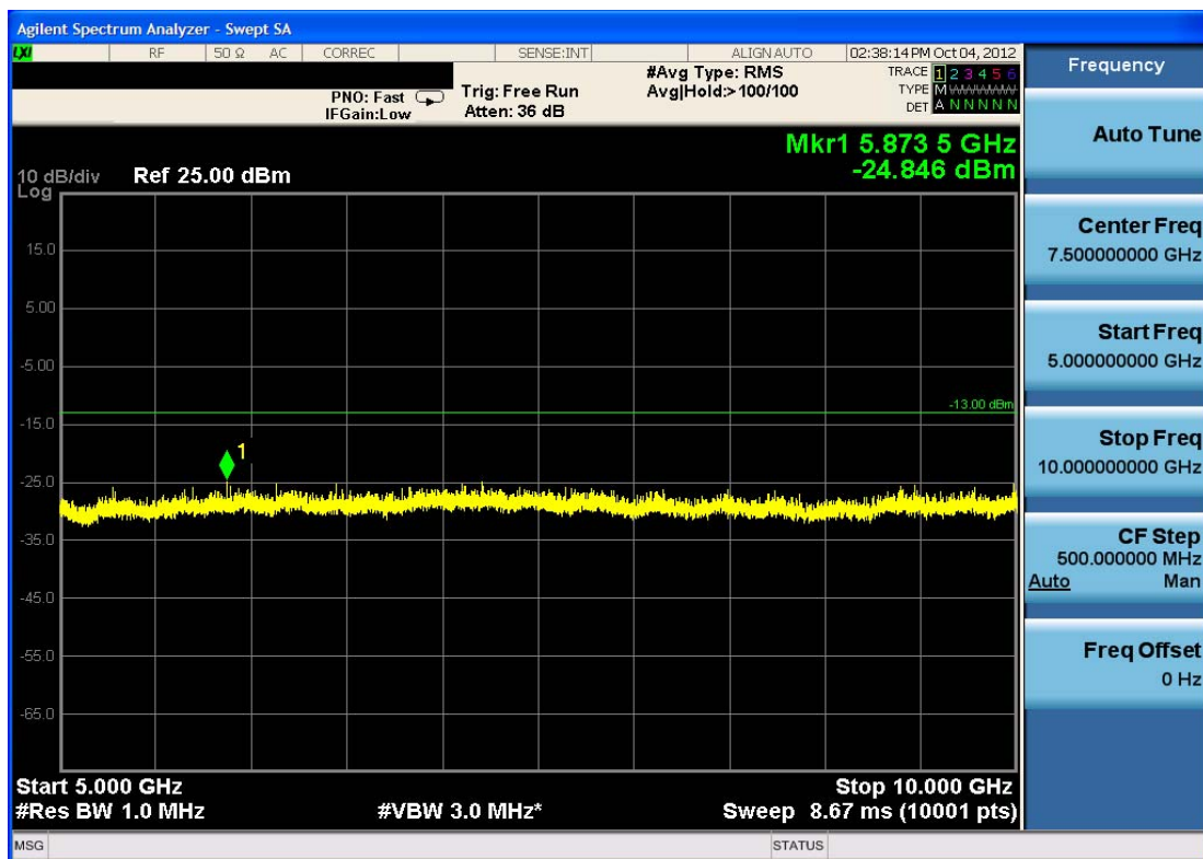
Plot 7-8. Conducted Spurious Plot (Cellular WCDMA Mode – Ch. 4183)
