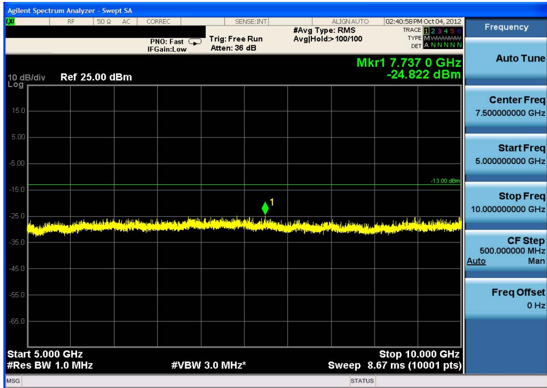
Plot 7-11. Conducted Spurious Plot (Cellular WCDMA Mode – Ch. 4233)
