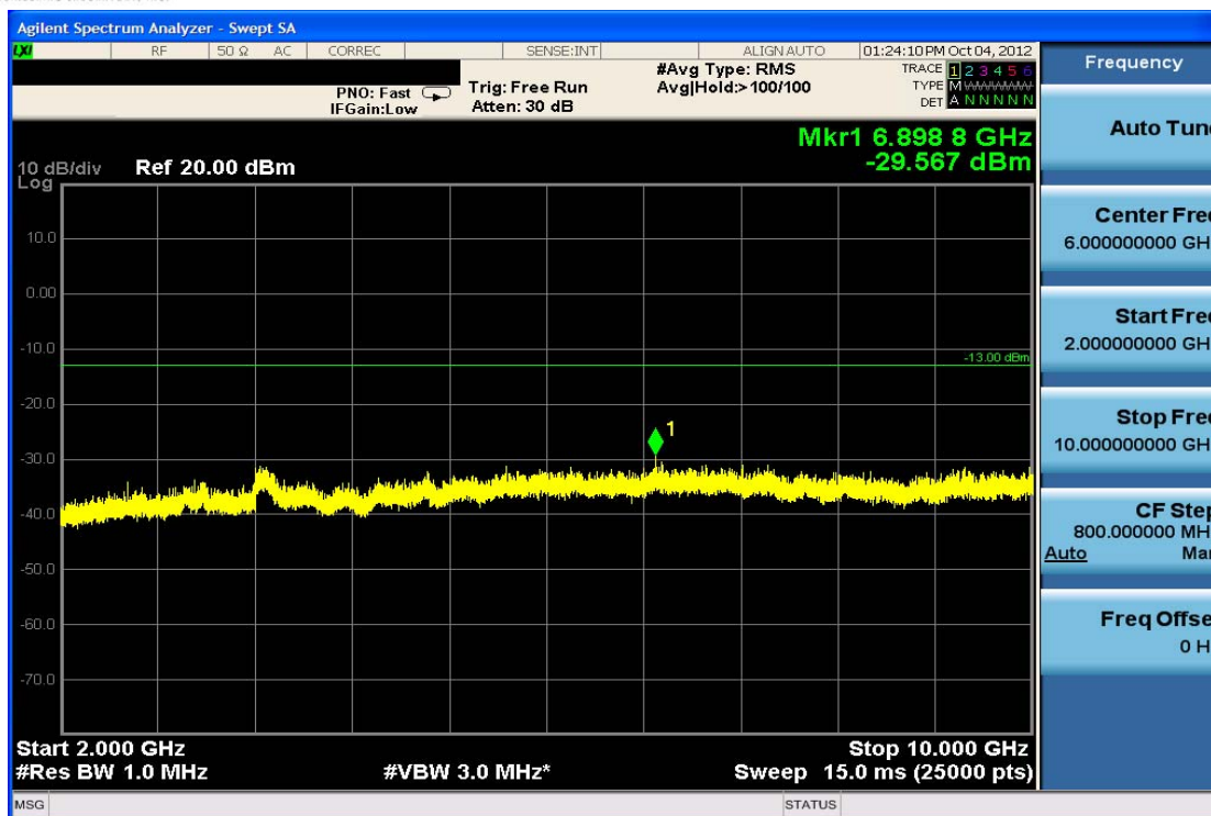
Plot 7-11. Conducted Spurious Plot (Cellular GSM Mode – Ch. 251)
