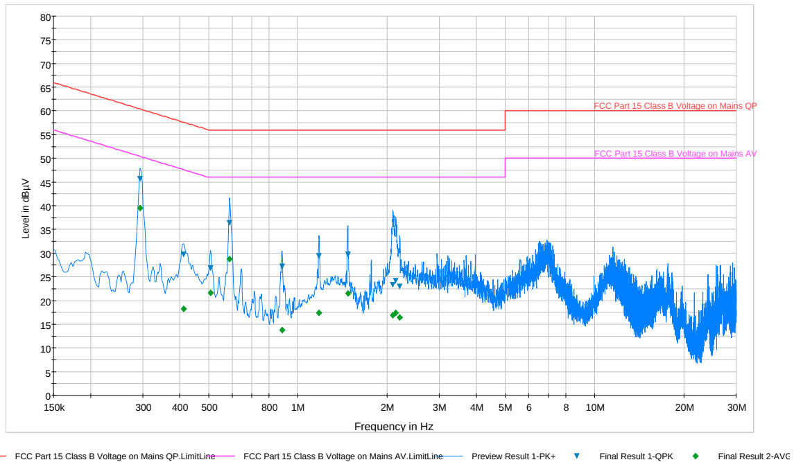
Plot 6-34. Line-Conducted Test Plot (N)
