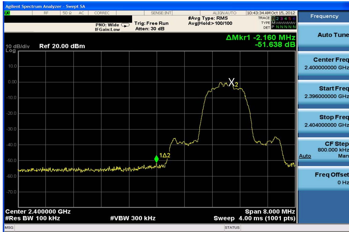
Plot 6-19. Band Edge Plot (Bluetooth with Hopping Disabled, 3Mbps – Ch. 0)
