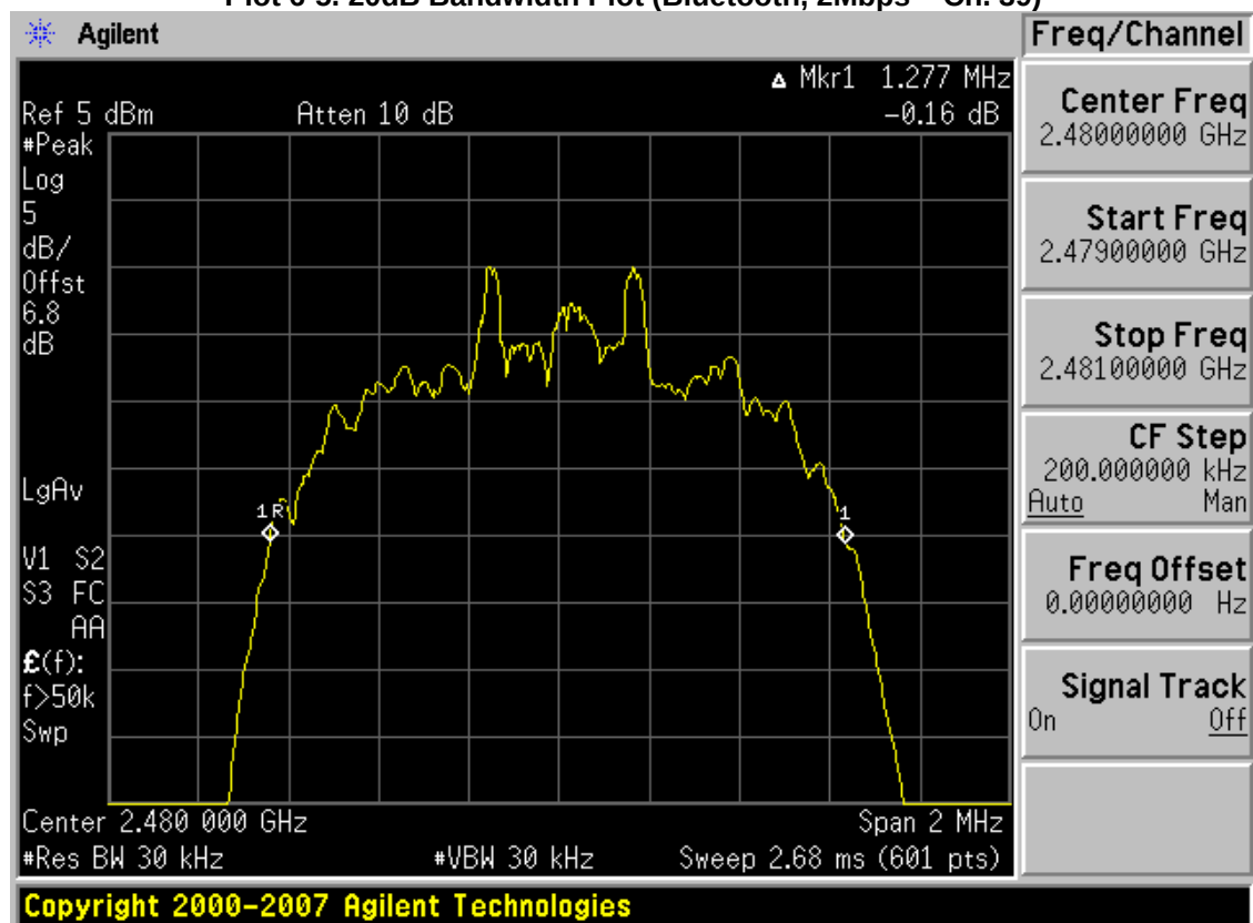
Plot 6-6. 20dB Bandwidth Plot (Bluetooth, 2Mbps – Ch. 78)
