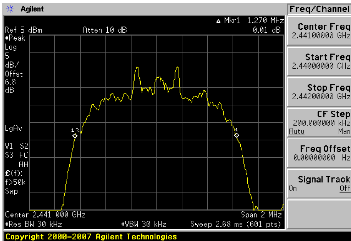
Plot 6-5. 20dB Bandwidth Plot (Bluetooth, 2Mbps – Ch. 39)
