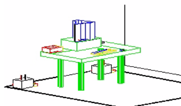
Figure 3-3. Wooden Table & Bonded LISNs
