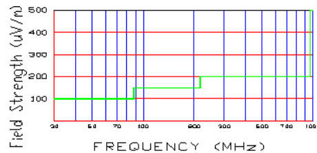
Figure A-8. Radiated limits at 3 meters.
