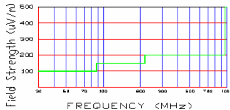
Figure A-9. Radiated limits at 3 meters.
