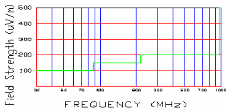
Figure A-7. Radiated limits at 3 meters.
