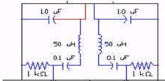
Figure 3.1-4. LISN Schematic Diagram
