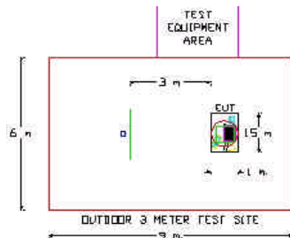
Figure 3.2-2. Dimensions of Outdoor Test Site
