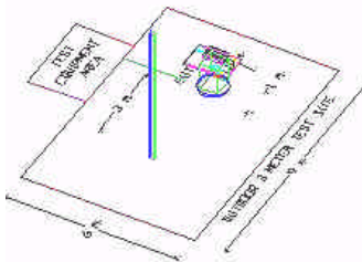
Figure 3.2-3. Turntable and System Setup
