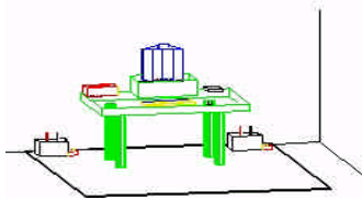
Figure 3.1-2. Line Conducted Emission Test Set-Up
