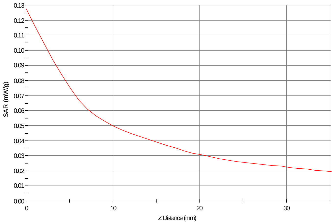
SAR - Z Axis at Hotspot x:89.0 y:-16.0
