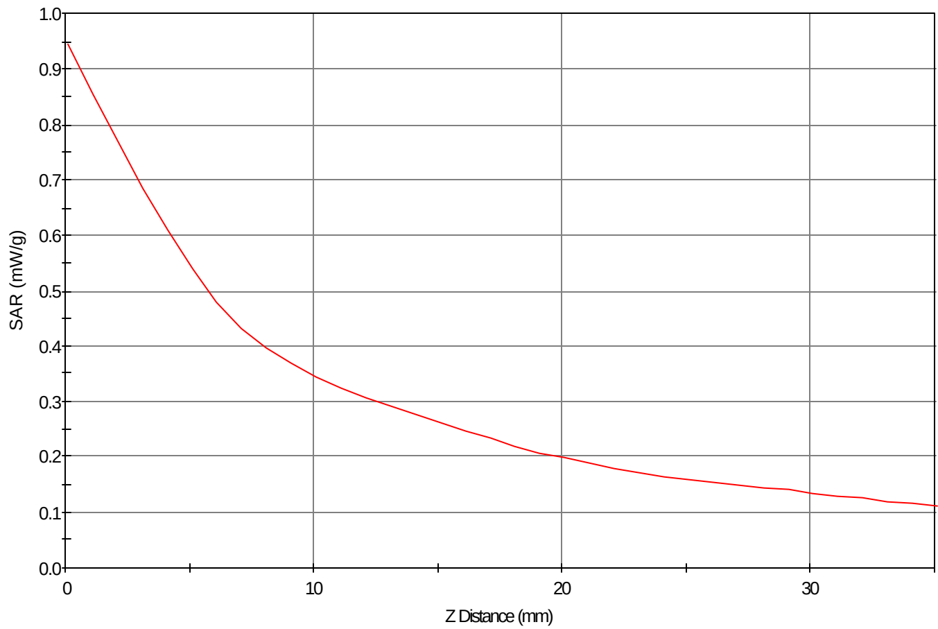
SAR - Z Axis at Hotspot x:109.0 y:11.0
