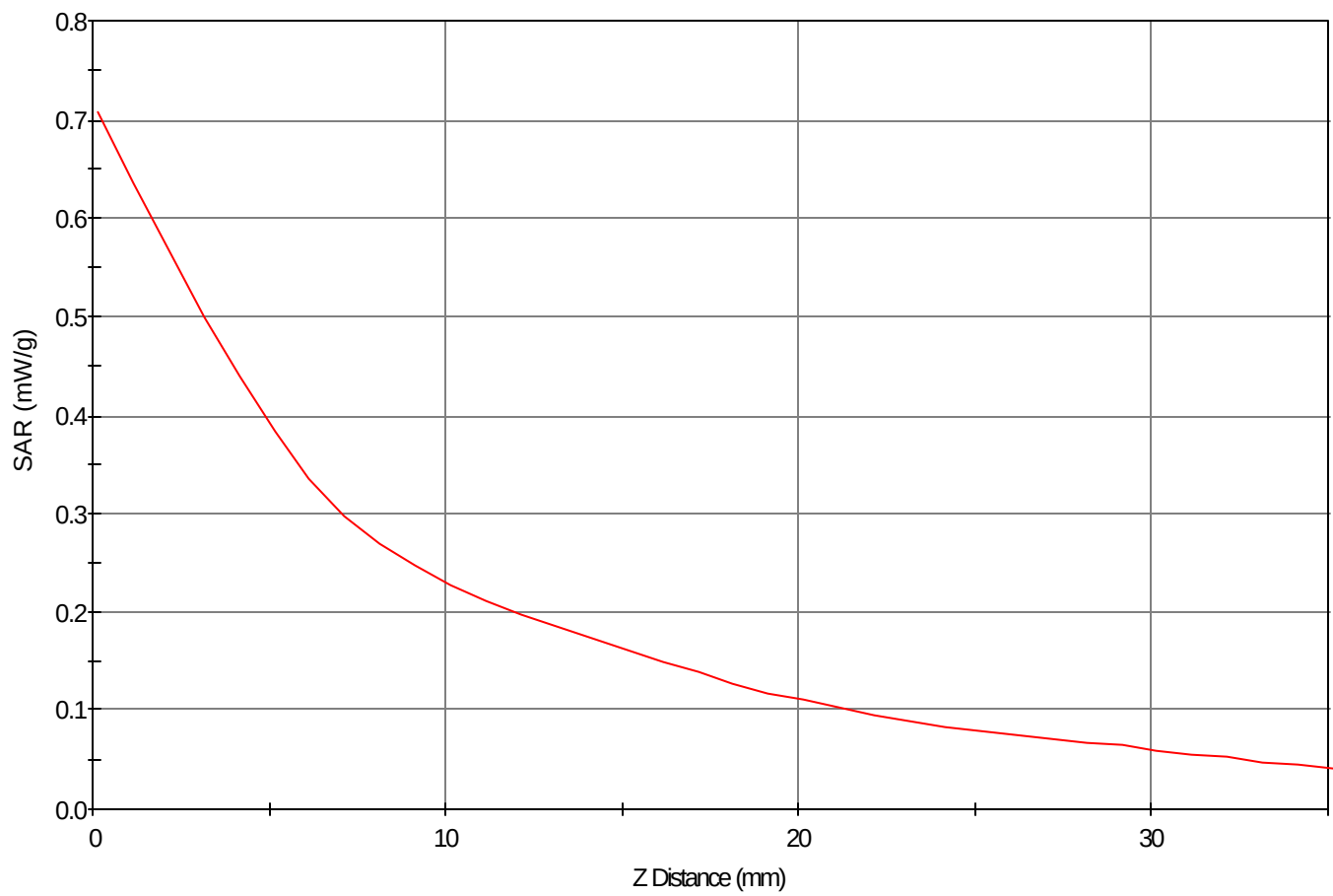
SAR - Z Axis at Hotspot x:14.0 y:-7.0
