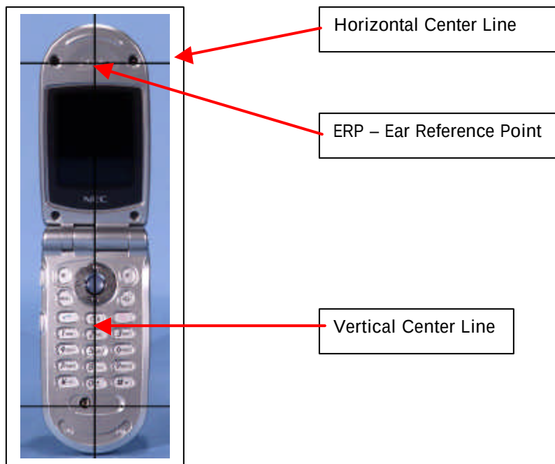
Figure 12.1 Handset Reference Points
