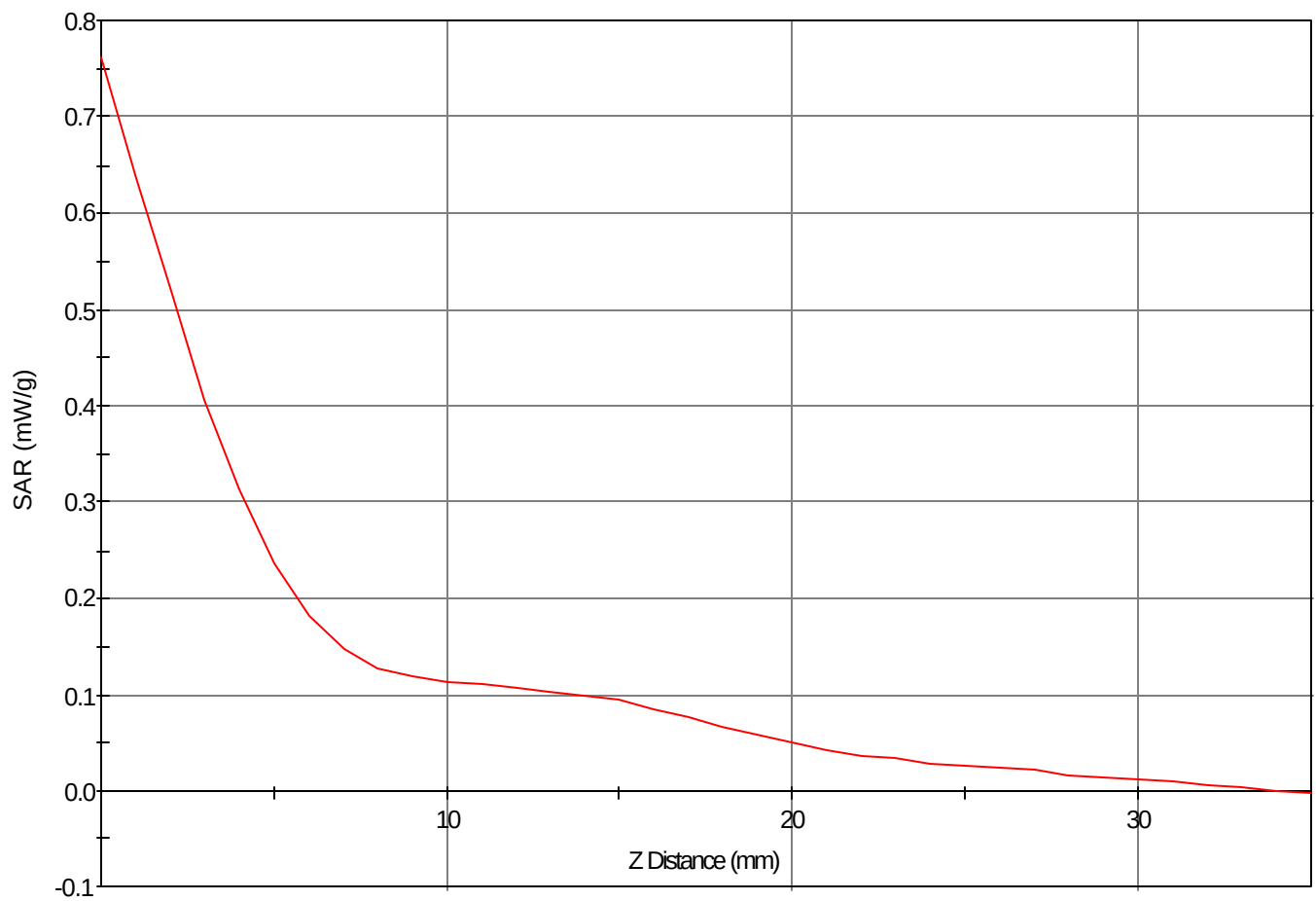
SAR - Z Axis at Hotspot x:90.0 y:0.0
