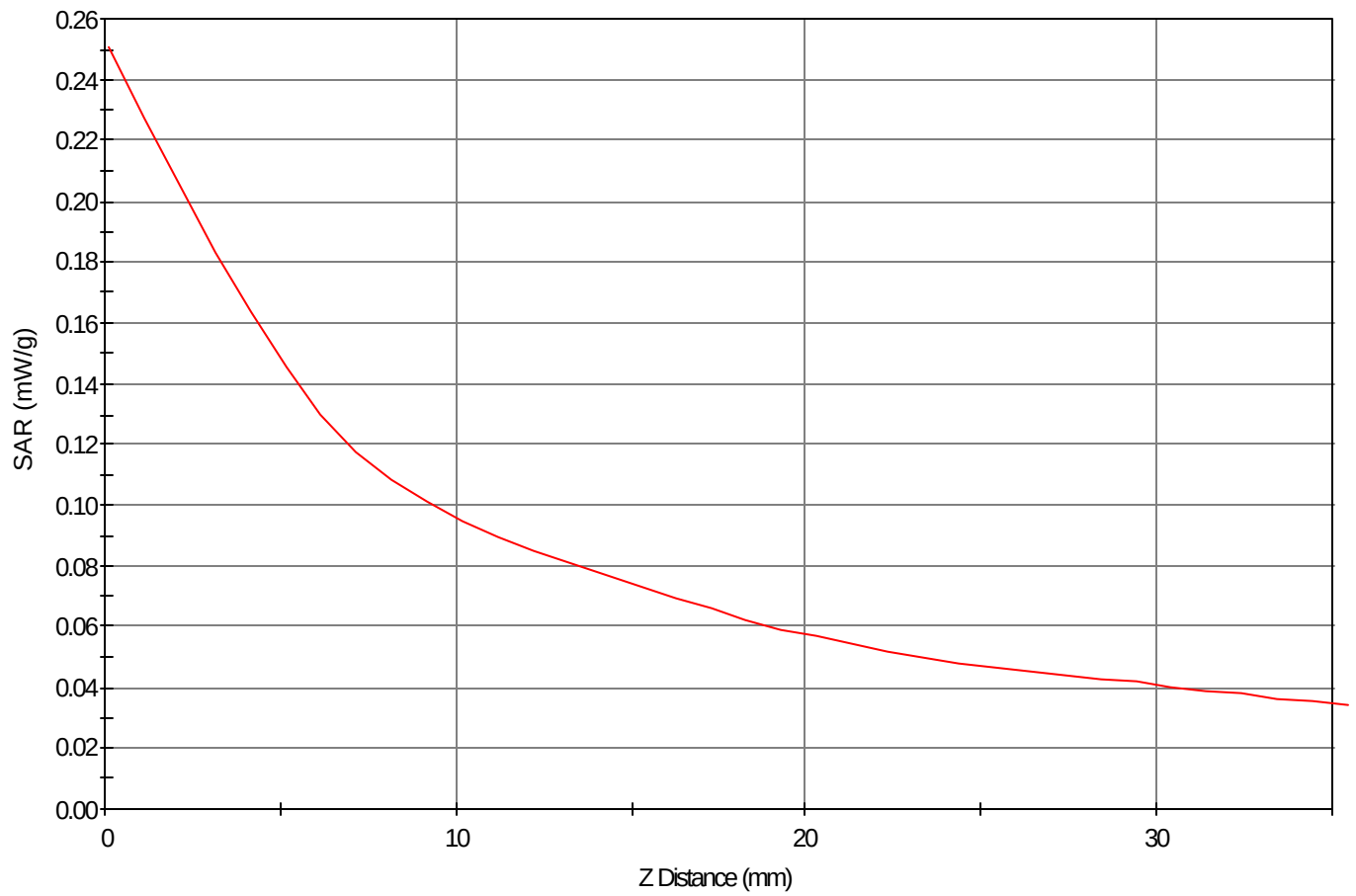
SAR - Z Axis at Hotspot x:101.0 y:-2.0
