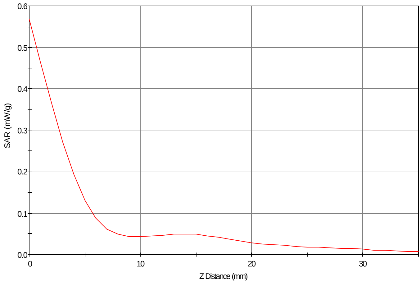
SAR - Z Axis at Hotspot x:104.0 y:19.0
