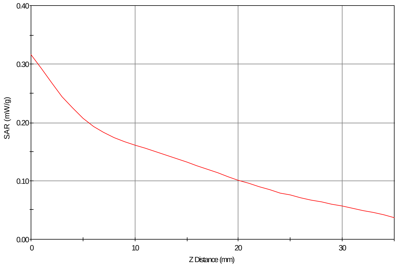
SAR - Z Axis at Hotspot x:90.0 y:1.0
