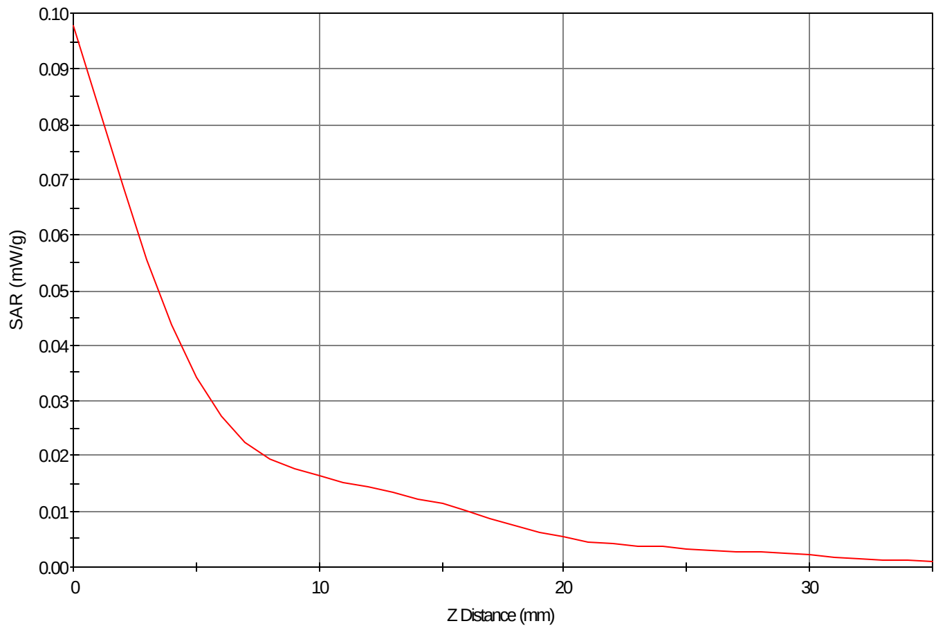
SAR - Z Axis at Hotspot x:95.0 y:-2.0
