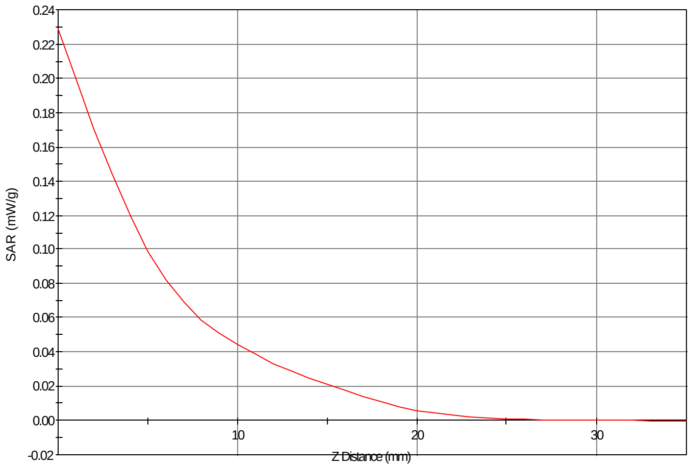
SAR - Z Axis at Hotspot x:5.0 y:-39.0
