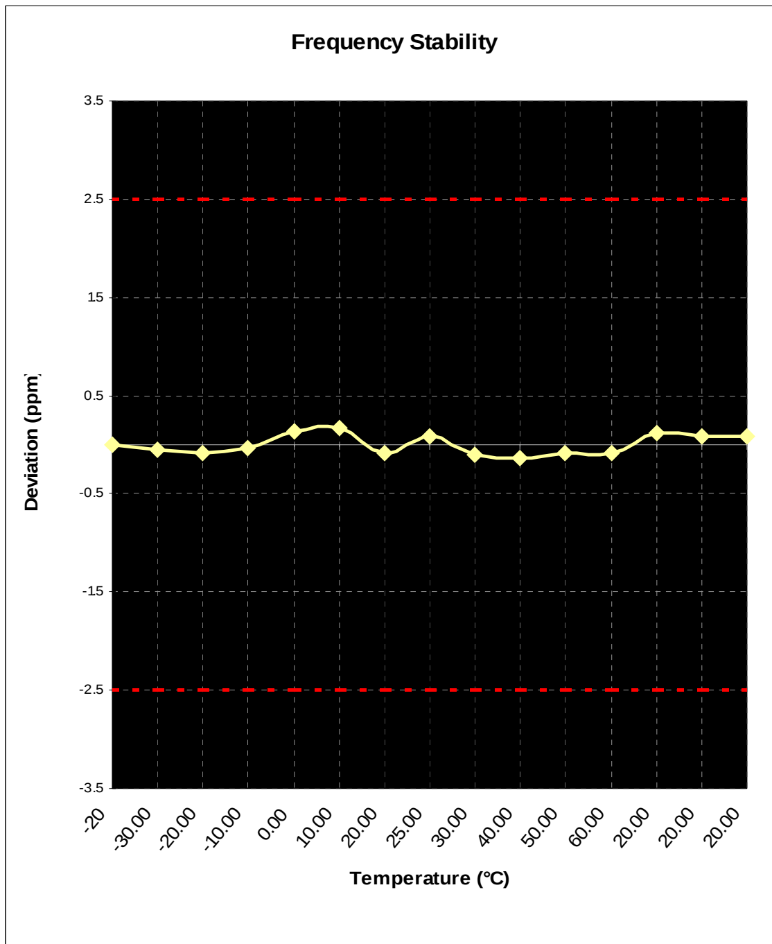
Plot 6-1. PCS GSM Frequency Deviation Graph
