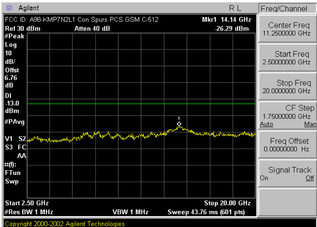
Plot A-2. Conducted Spurious (PCS GSM – Ch. 512)
