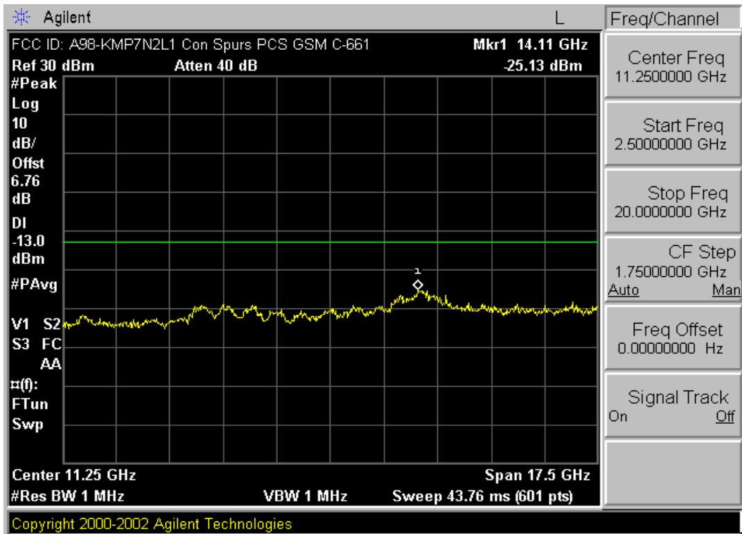
Plot A-5. Conducted Spurious (PCS GSM – Ch. 661)
