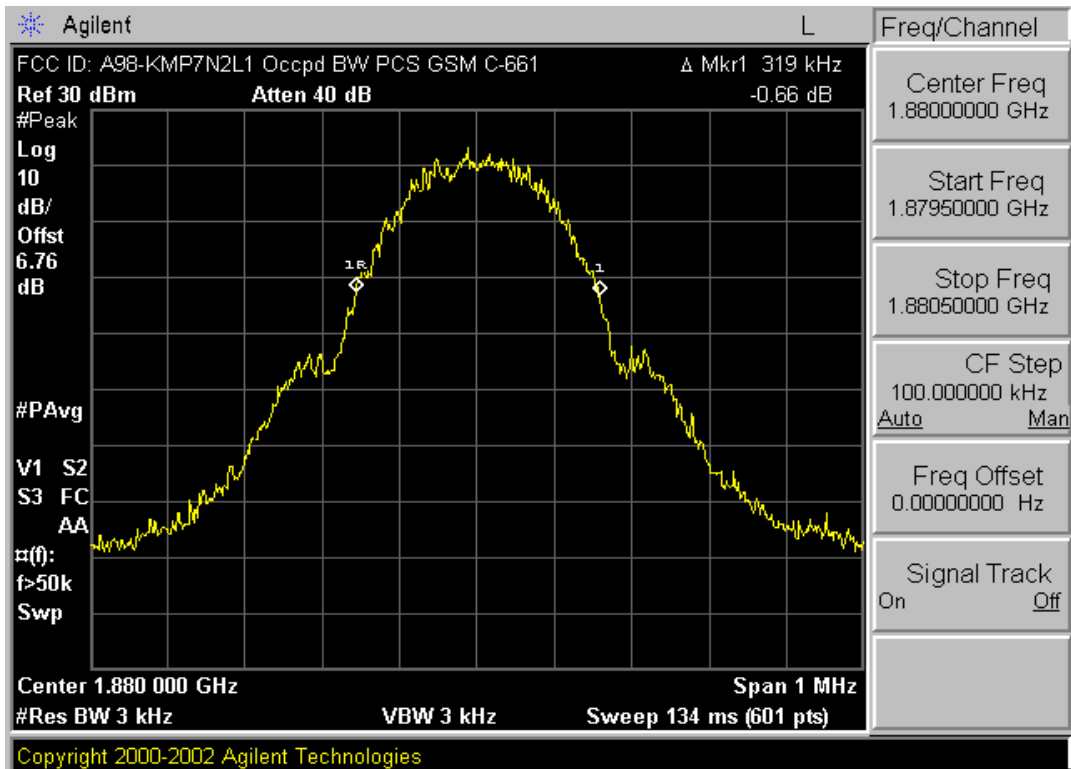
Plot A-6. Occupied Bandwidth (PCS GSM – Ch. 661)
