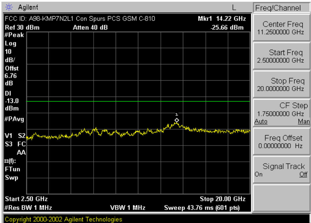
Plot A-8. Conducted Spurious (PCS GSM – Ch. 810)
