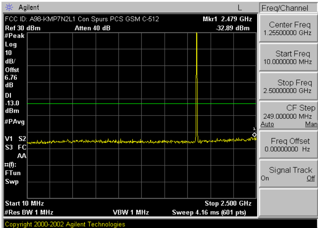
Plot A-1. Conducted Spurious (PCS GSM – Ch. 512)
