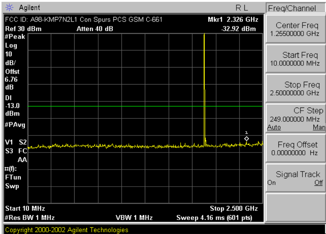
Plot A-4. Conducted Spurious (PCS GSM – Ch. 661)
