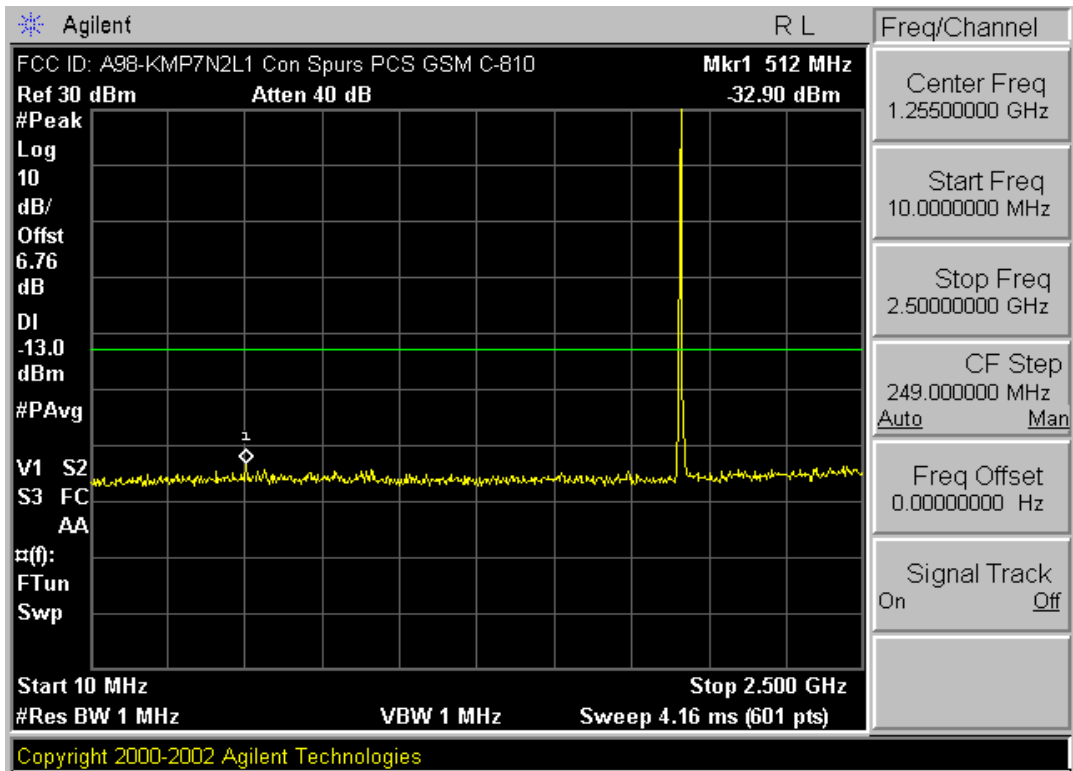
Plot A-7. Conducted Spurious (PCS GSM – Ch. 810)
