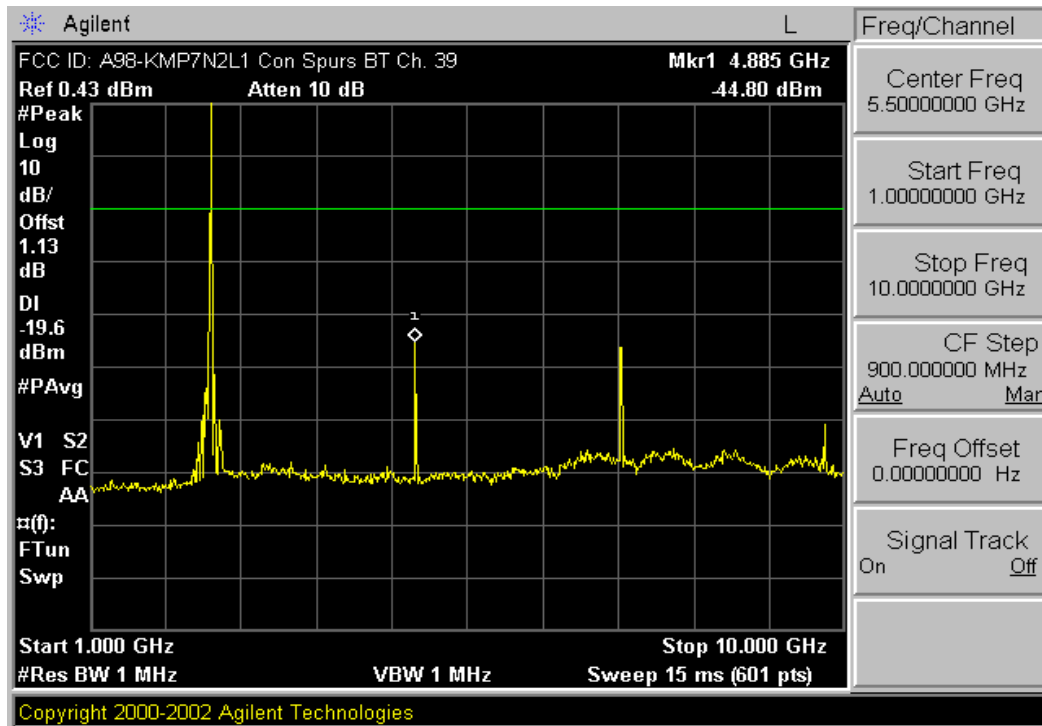
Plot 6-12. Conducted Spurious Plot (Bluetooth – Ch. 39)
