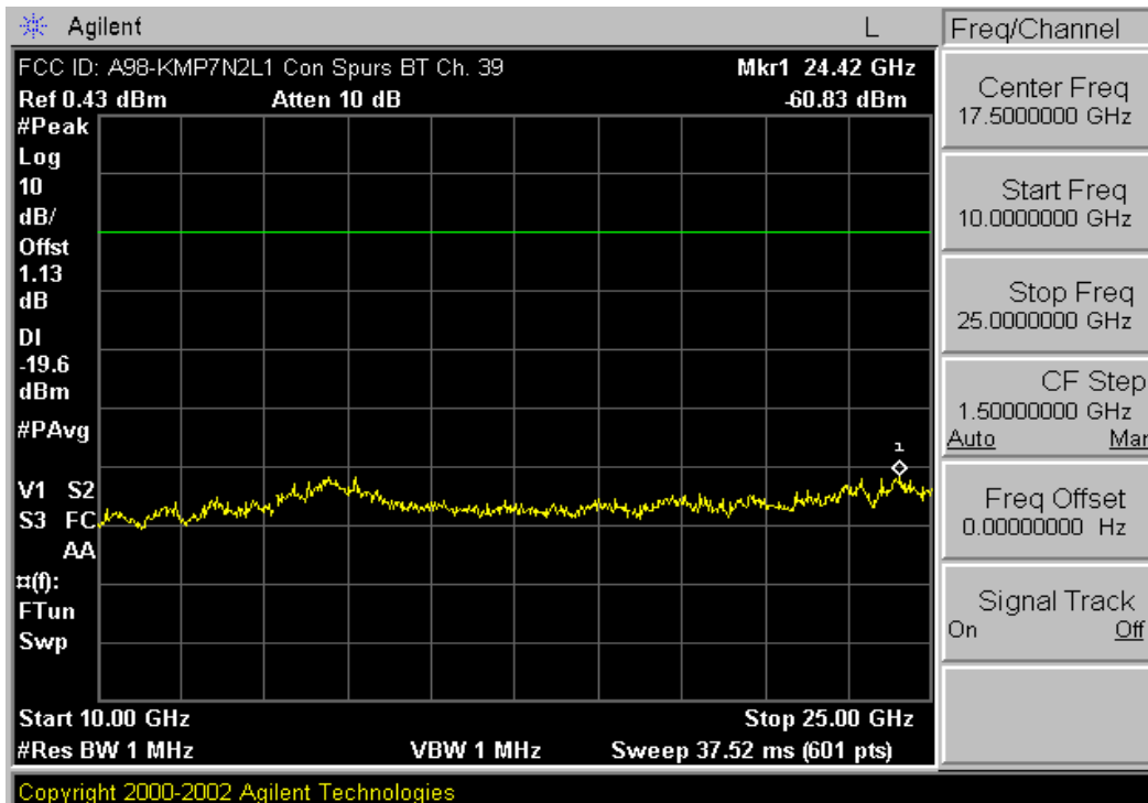
Plot 6-13. Conducted Spurious Plot (Bluetooth – Ch. 39)
