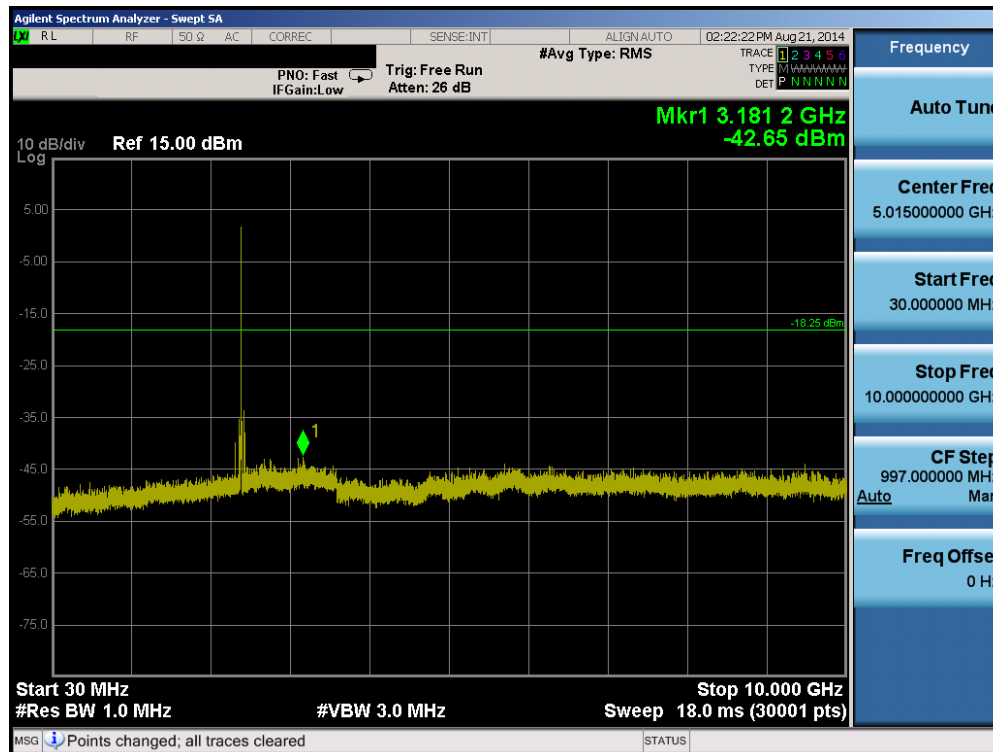
Plot 6-14. Conducted Spurious Plot (Bluetooth (LE) – Ch. 0)
