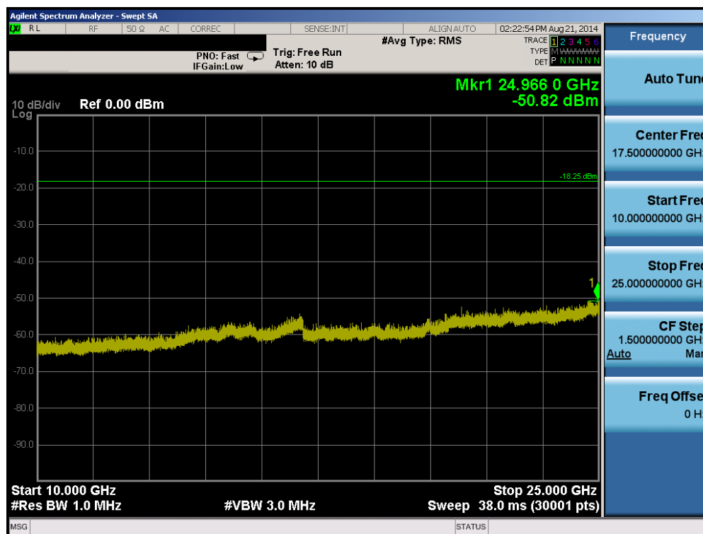
Plot 6-15. Conducted Spurious Plot (Bluetooth (LE) – Ch. 0)
