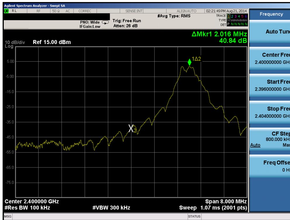
Plot 6-10. Band Edge Plot (Bluetooth (LE) with Hopping Disabled – Ch. 0)
