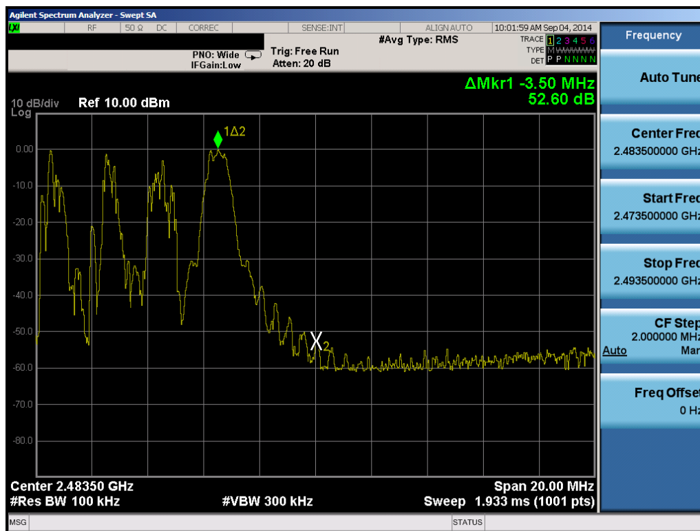
Plot 6-13. Band Edge Plot (Bluetooth (LE) with Hopping Enabled – Ch. 39)
