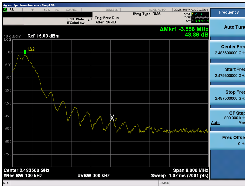
Plot 6-11. Band Edge Plot (Bluetooth (LE) with Hopping Disabled – Ch. 39)
