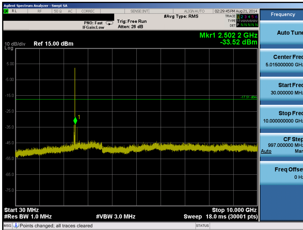
Plot 6-18. Conducted Spurious Plot (Bluetooth (LE) – Ch. 39)
