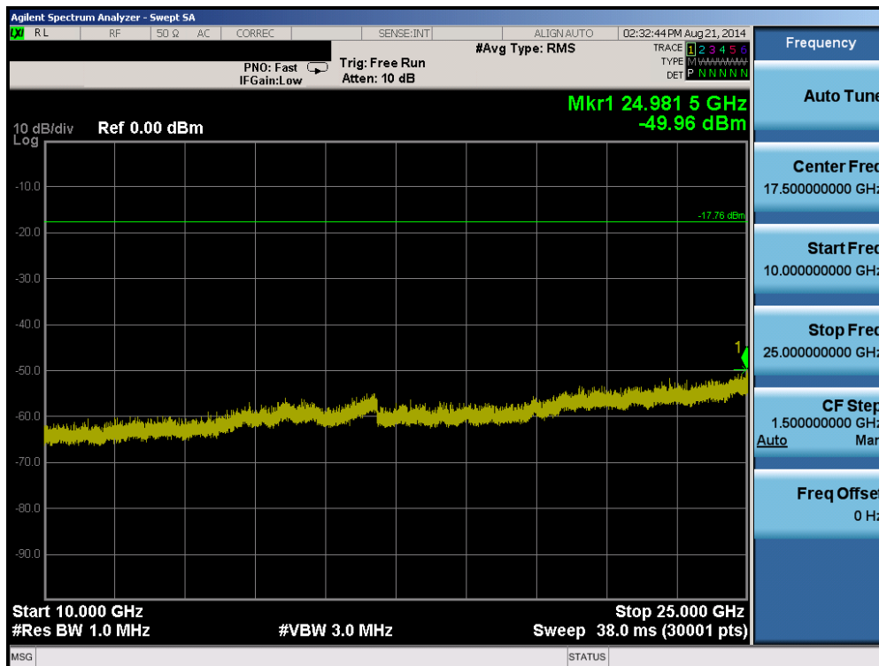
Plot 6-17. Conducted Spurious Plot (Bluetooth (LE) – Ch. 19)
