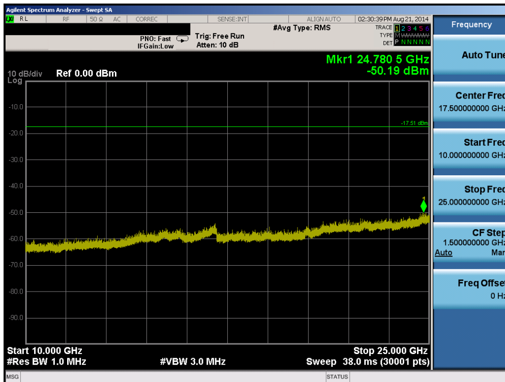
Plot 6-19. Conducted Spurious Plot (Bluetooth (LE) – Ch. 39)
