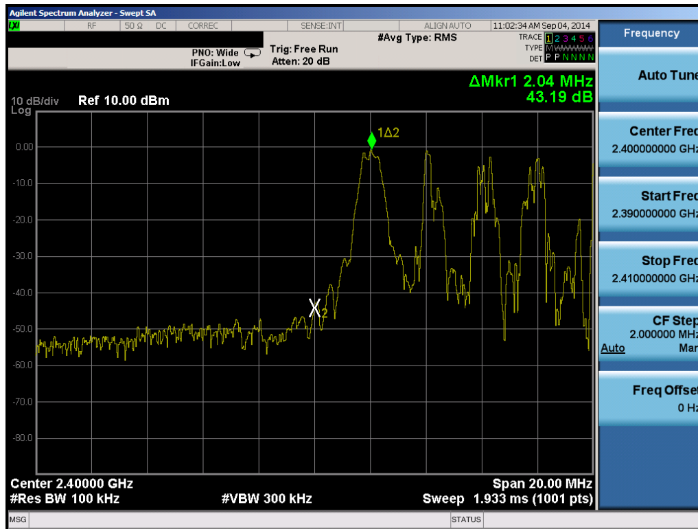
Plot 6-12. Band Edge Plot (Bluetooth (LE) with Hopping Enabled – Ch. 0)
