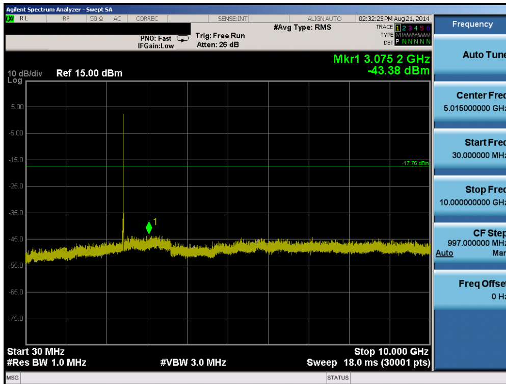
Plot 6-16. Conducted Spurious Plot (Bluetooth (LE) – Ch. 19)
