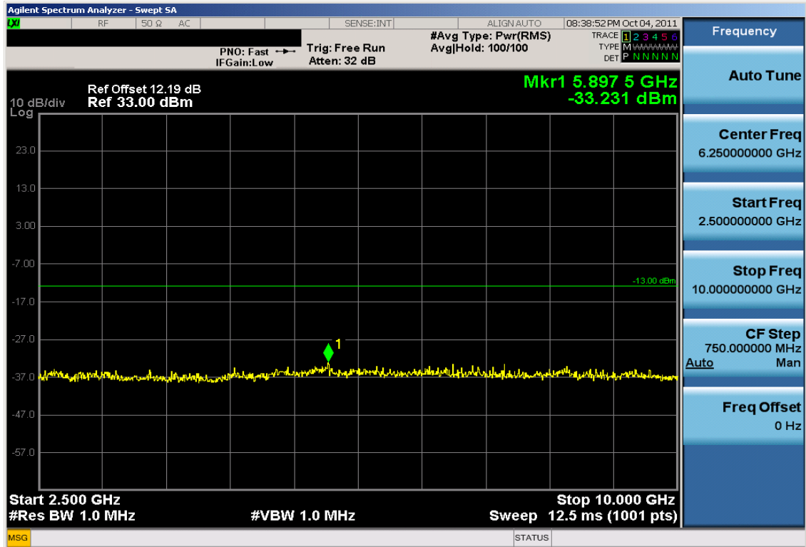
Plot 7-25. Conducted Spurious Plot (Cellular WCDMA Mode – Ch. 4183)
