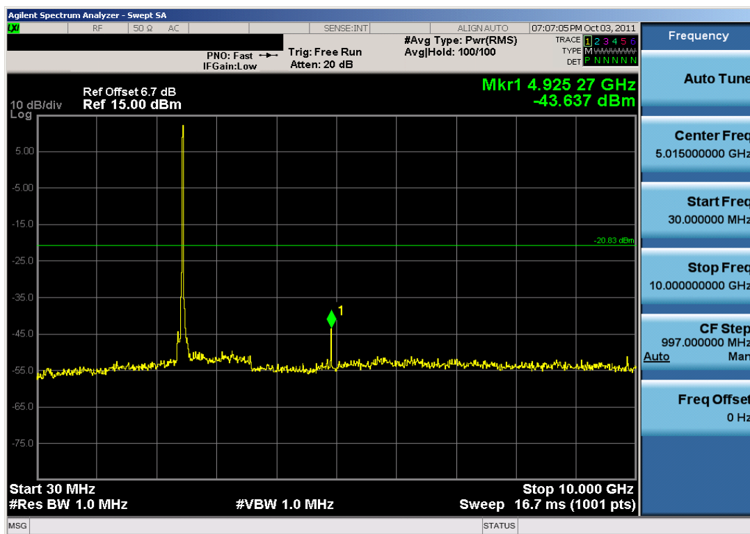
Plot 6-29. Conducted Spurious Plot (802.11b – Ch. 11)
