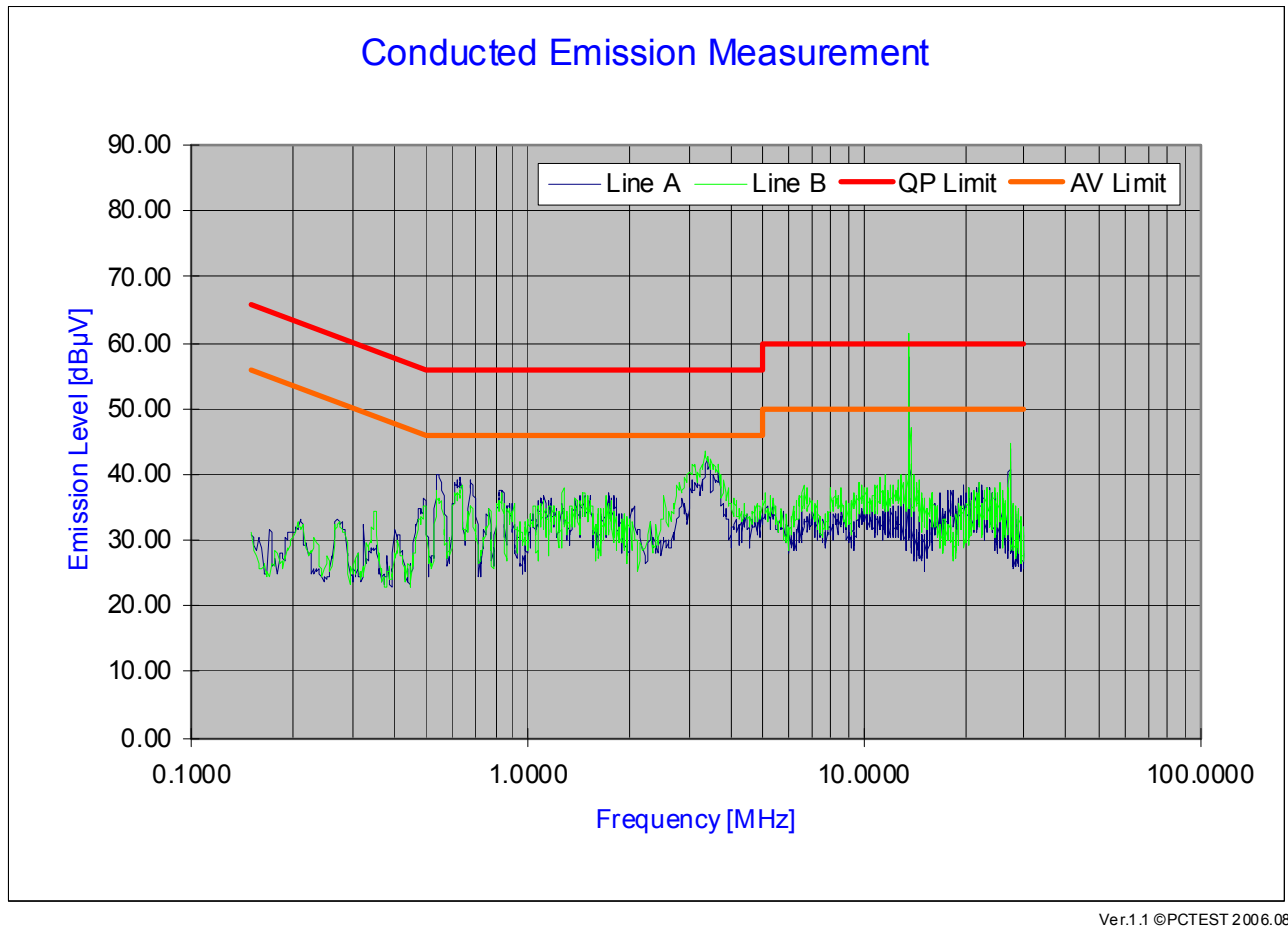
Plot 8-1. Line-Conducted Test Plot
