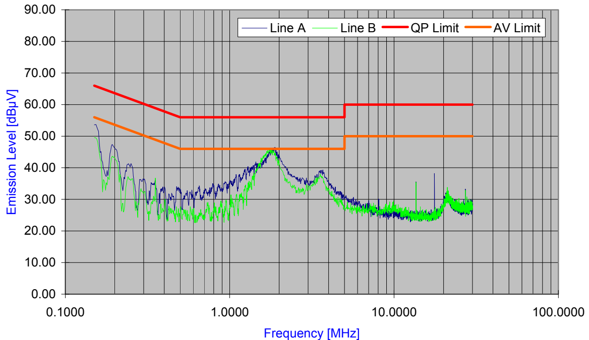
Plot 8-2. Line-Conducted Test Plot
